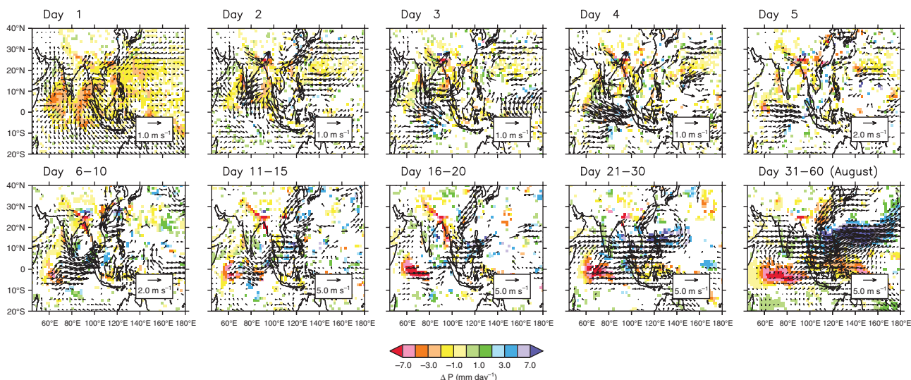
Figure 10. As Figure 9, but for the global initialised experiment. The reference wind speed increases from 1 to 5 \text{m s}^{-1} through the panels and is not always the same as the reference wind speed in Figure 9.
