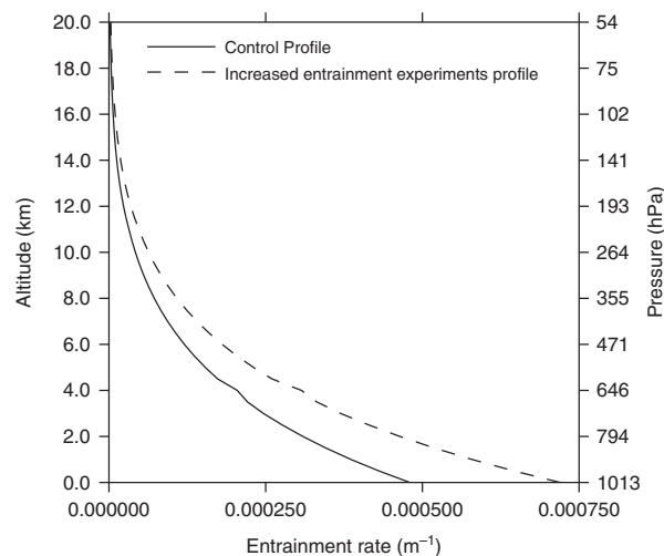
Figure 2. The fractional mixing entrainment rate profile for mid-level and deep convection in the configuration of the MetUM used in this study. The solid (dashed) line is the default (increased) profile for an ICAO standard atmosphere.
