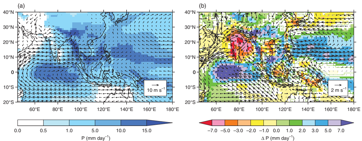
Figure 1. (a) JJAS precipitation (shading, mm day -1 ) and 850 hPa winds (arrows, m s -1 ) in our control integration (section 2). (b) Bias with respect to GPCP precipitation and ERA-Interim 850 hPa winds. Shaded grid points in (b) indicate precipitation biases are significant at the 95% level using a Student's t -test, less significant changes are outlined. Black (grey) arrows indicate either the zonal or meridional wind biases are significant (not significant) at the 95% level.
