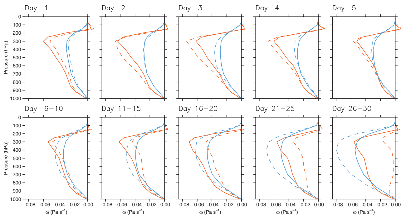
Figure 13. Evolution of 20-year mean profiles of \omega \text{ (Pa s}^{-1}\text{)} in the control (solid lines) and global initialised experiment (dashed lines) averaged over the WEIO (red) and WNP (blue). This figure is available in colour online at wileyonlinelibrary.com/journal/qj
