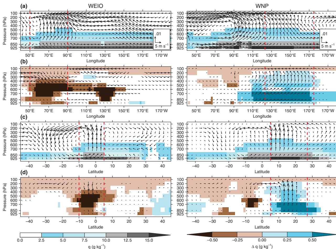
Figure 18. (a) JJAS specific humidity (shading, g\ kg^{-1} ) and zonal circulation (arrows, m\ s^{-1} ) meridionally averaged across the WEIO and WNP in the control integration. (b) Changes in the global AMIP-style experiment. Only changes significant at a 95% level with a Student's t -test are shown. (c, d) are as (a, b) but for meridional circulation zonally averaged. Although these are for the global experiment, the red dashed lines denote the boundaries of the WEIO and WNP regions for reference.
