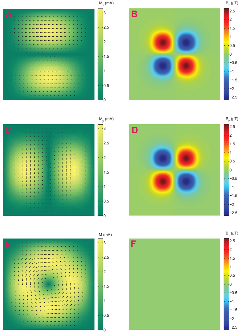
FIGURE 1. Example of a silent source magnetization defined by \mathbf{m}(x, y) = (\psi(x)\psi'(y), -\psi'(x)\psi(y), 0) where \psi(t) := (1/2)(1 - \cos(2\pi t)) for t \in [0, 1] and is zero otherwise. Parts A and B show the magnetization \mathbf{m}_1(x, y) = (\psi(x)\psi'(y), 0, 0) and resulting vertical component of the magnetic field measured at height z = 0.1 mm. Parts C and D show the magnetization \mathbf{m}_2(x, y) = (0, -\psi'(x)\psi(y), 0) and resulting vertical component of the magnetic field measured at height z = 0.1 mm. Parts E and F illustrate the silent source magnetization \mathbf{m} = \mathbf{m}_1 + \mathbf{m}_2 and resulting null vertical component of the magnetic field measured at height z = 0.1 mm. Each image corresponds to an area of 1 \text{ mm} \times 1 \text{ mm} .
