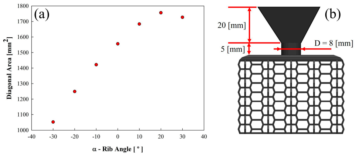
Figure 2. (a) Model selection by diagonal area analysis and (b) gating and selected model detail.
