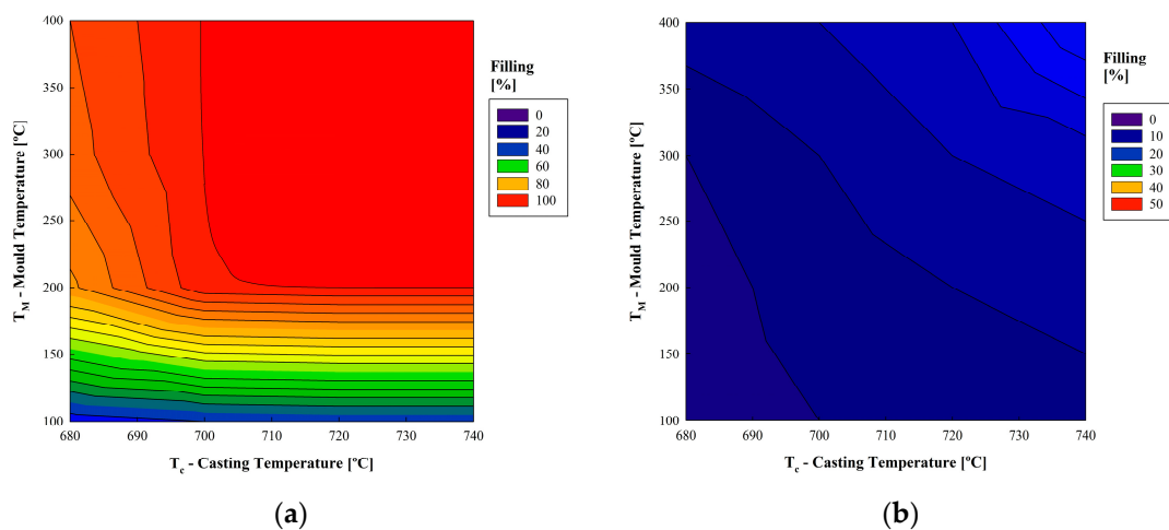
Figure 6. Average sample filling using different combinations of mold and casting temperatures: (a) with vacuum; and (b) without vacuum.
