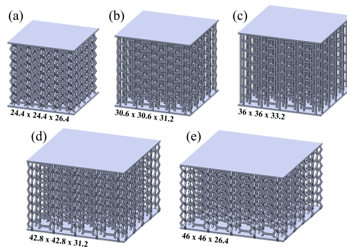
Figure 1. CAD models for scaffold models (dimensions in mm), with rib angles: (a) −30°; (b) −20°; (c) 0°; (d) 20° and (e) 30°.
