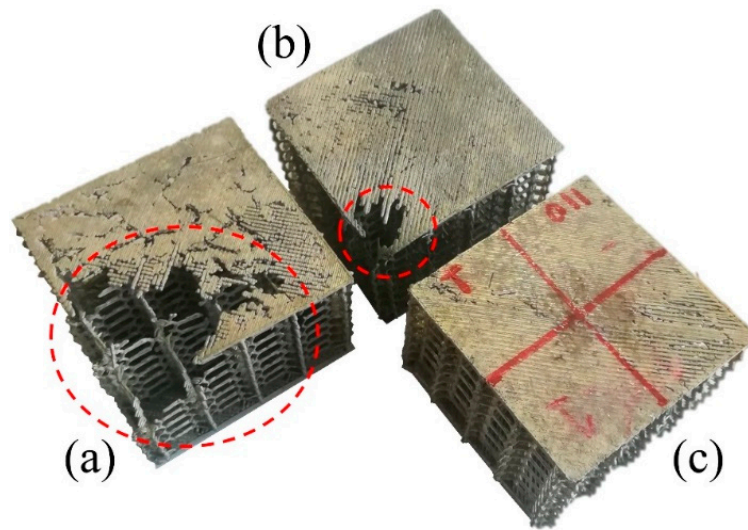
Figure 5. Characterization of average filling using different temperatures using vacuum assistance: (a) 83% ( \pm 6.3\% )— T_M = 200\text{ }^\circ\text{C} and T_C = 680\text{ }^\circ\text{C} ; (b) 92% ( \pm 4.1\% )— T_M = 200\text{ }^\circ\text{C} and T_C = 700\text{ }^\circ\text{C} ; and (c) complete filling— T_M = 250\text{ }^\circ\text{C} and T_C = 700\text{ }^\circ\text{C} .
