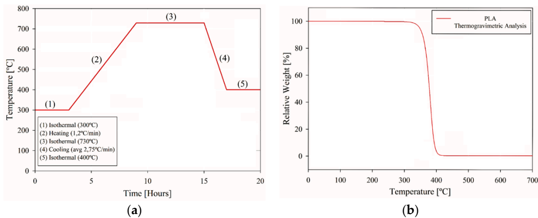
Figure 3. Ceramic block manufacturing: (a) mold thermal cycle; (b) PLA thermogravimetric analysis.
