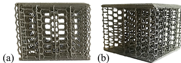
Figure 4. Developed manufacturing process as-cast sample ( T_M = 250 °C and T_C = 700 °C, using vacuum assistance): (a) front and (b) corner views.
