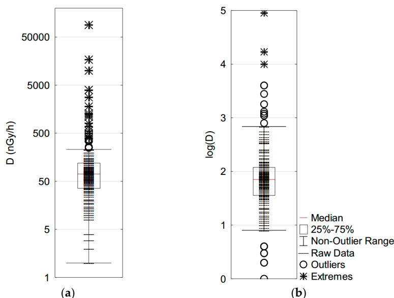
Figure 3. Boxplots of set of absorbed dose rate values from Reference [1] corresponding to minimum values, average values, and maximum values by country as well as values from areas with high natural gamma radiation background: (a) original values and (b) logarithms of original values.
