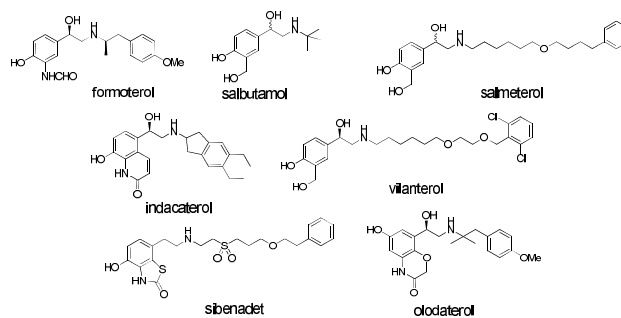
Figure 1: A selection of known \beta_2 AR agonists and sibenadet - a dual D 2 dopamine receptor, \beta_2 -AR agonist.
