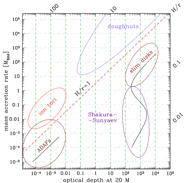
Fig. 1. This figure illustrates a few of the most well-known analytic and semi-analytic solutions of the stationary black hole accretion disks. Their location in the parameter space approximately corresponds to viscosity \alpha = 0.1 and radius r = 20 M .
