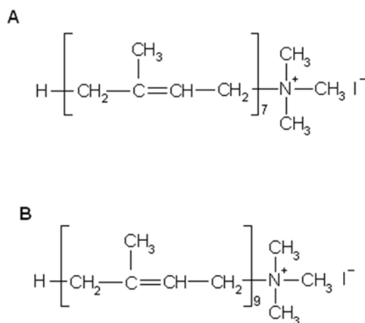
Figure 1. Structures of heptaprenyltrimethylammonium (A) and nonaprenyltrimethylammonium (B) iodides.
