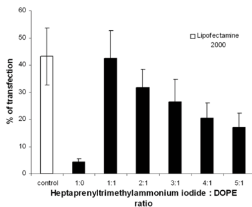
Figure 4. The effect of heptaprenyltrimethylammonium iodide : DOPE ratio on transfection efficiency.
