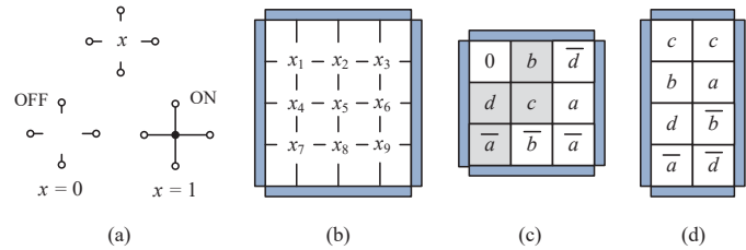
Fig. 1. (a) Four-terminal switch; (b) 3 \times 3 four-terminal switching network; realizations of f = \overline{a}bcd + a\overline{b}cd : (c) using the 3 \times 3 switching lattice; (d) using a switching lattice with the minimum size, i.e., 4 \times 2 .
