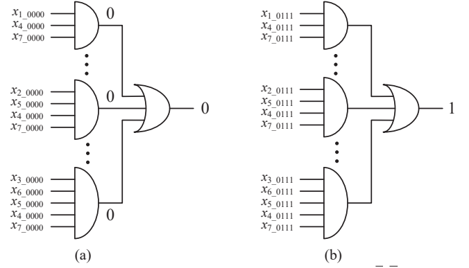
Fig. 3. The combinational circuits of f_{3 \times 3} for f = \bar{a}bcd + \bar{a}\bar{b}c\bar{d} : (a) when abcd = 0000 and f is low; (b) when abcd = 0111 and f is high.
