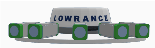
Fig. 3: Sketch of the sensor platform. The five camera houses are looking forward. Camera units, CW-FM RADAR and GPS receiver are mounted on the test platform. The combined horizontal field of view of two daylight cameras is 110 deg.
