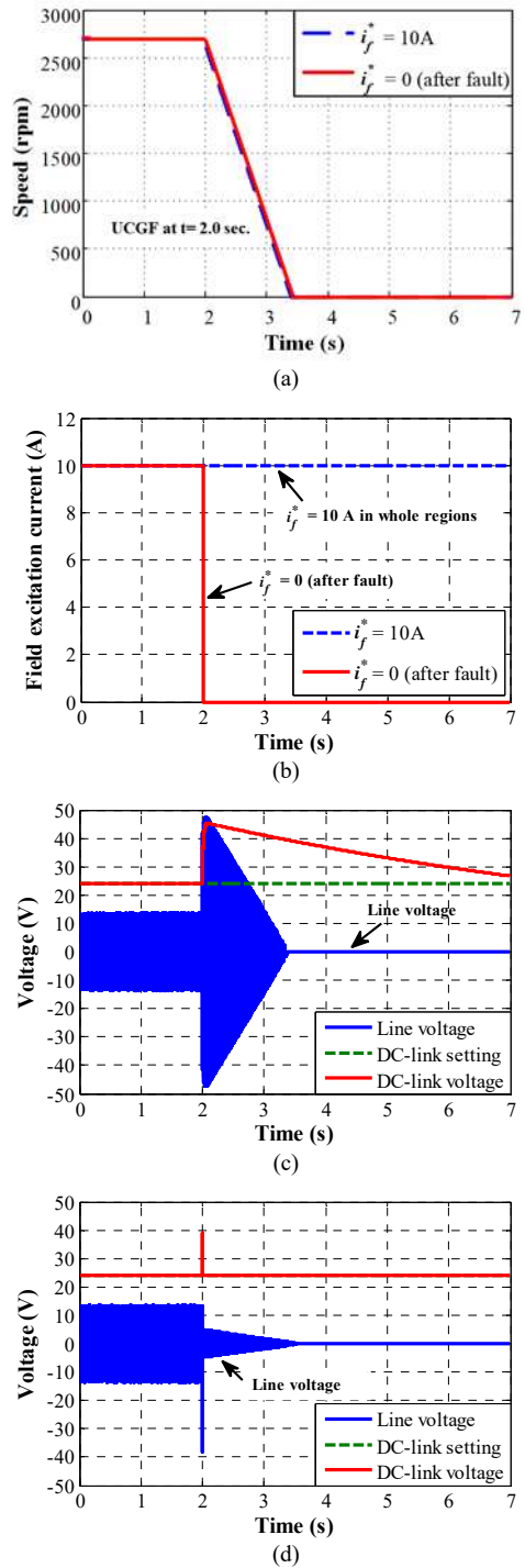
Fig. 7. Simulation results of the proposed fault protection method ( i_f^* = 0 ) compared to the method utilizing the maximum field excitation current for all regions ( i_f^* = 10\text{ A} ). (a) Speed, (b) Field excitation current control, (c) Line voltage ( i_f^* = 10\text{ A} ), (d) Line voltage ( i_f^* = 0 after UCGF).
