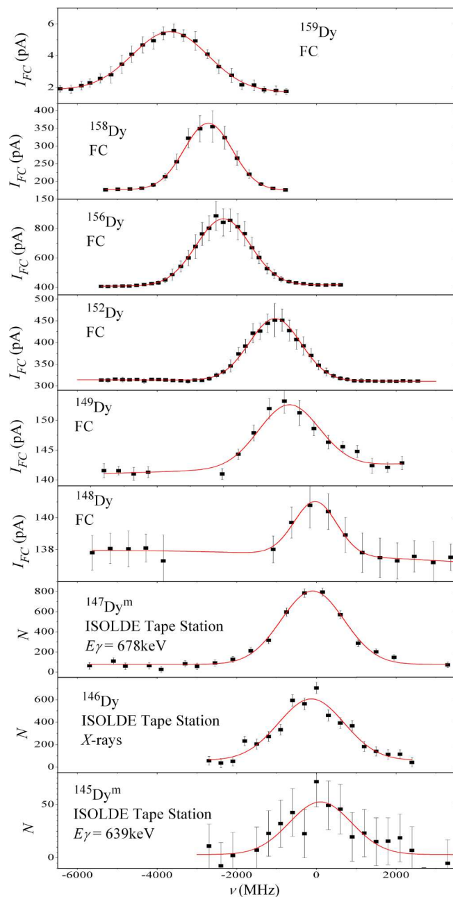
Fig. 1. Spectra for ^{159,158,156,152,149,148,147m,146,145m}\text{Dy} isotopes. For the odd-A dysprosium isotopes, the resolution was not high enough to resolve the HFS and therefore only the isotope shifts were extracted. The shift in center of gravity (CoG), introduced by the underlying HFS for these cases, was taken into account by estimating it with reasonable A and B HFS-constants: A - and B -constants ratios for the excited and ground states were taken from [9], for ^{159,148,147m}\text{Dy} the known Q and \mu values [10] were used to calculate A and B constants by the standard scaling relation [11], \mu ( ^{145m}\text{Dy} ) and Q ( ^{145m}\text{Dy} ) were set to be equal to the corresponding values for ^{147m}\text{Dy} with the same shell-model configuration ( \nu h_{11/2} ). The shift proved to be less than \sim 40 MHz and was added to the uncertainties of the IS for the odd Dy isotopes.
