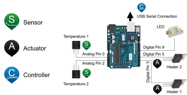
Fig. 3. Temperature sensors and heater actuators with connections to an Arduino.
