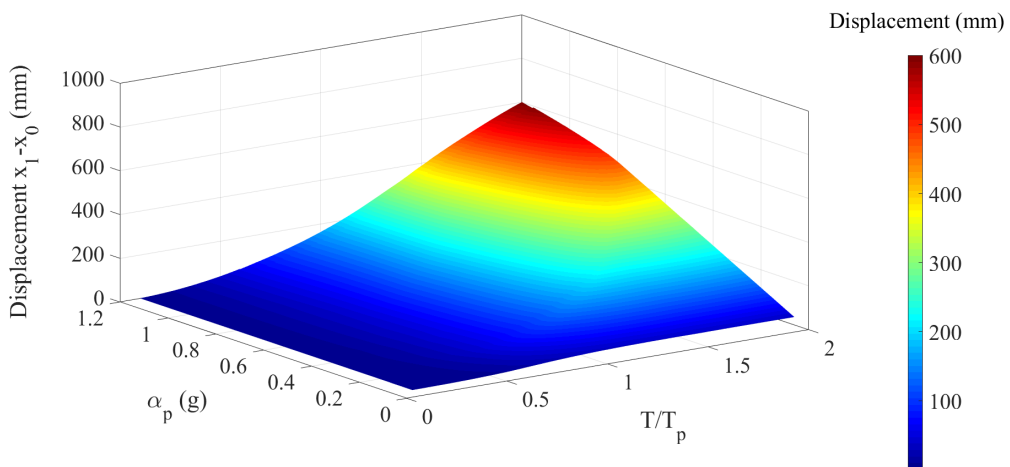
Fig. 15. Maximum displacement values of the structure (in mm) subjected to analytical Ricker pulse ground motion with varying a_p (g) and for different vibration period ratios T/T_p for a rigid sliding layer.
