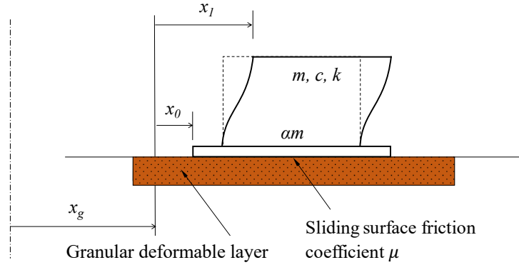
Fig. 1. Modelling of a flexible structure founded on a deformable granular layer.
