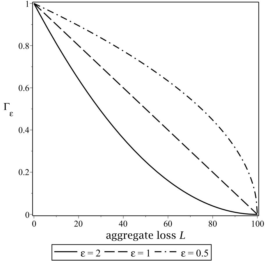
Figure 1: Graph of the Gamma Function for \Omega = 100
