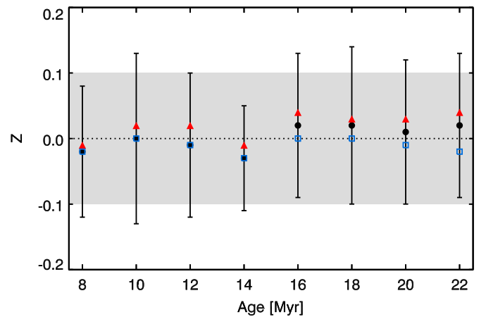
Figure 4. Metallicities extracted from synthetic SSC spectra as a function of age. Black circles show values extracted from the spectra when a 5% flat contaminative flux is removed from each spectra, red triangles are a result of the RSG population alone, and blue squares show metallicities extracted from the full spectra. Error bars on the black circles are consistent for each of the three types of measurement. The gray zone is the expected region of uncertainty for a single solar metallicity analyzed with the method used in this paper and initially presented by Davies et al. (2010) and Gazak et al. (2014).
