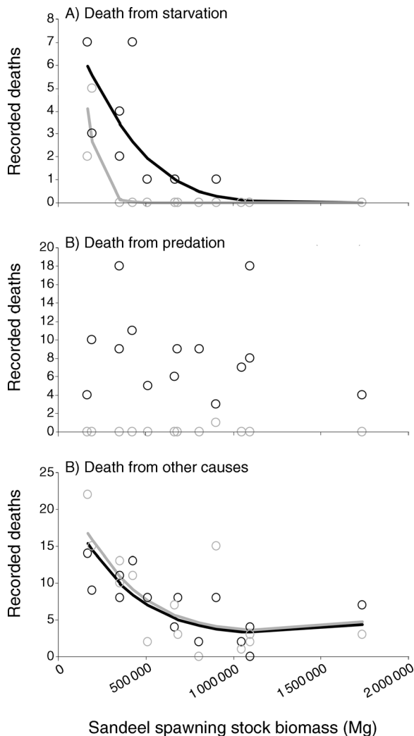
FIG. 4. Prey abundance and recorded mortality. Sandeel spawning stock biomass (measured in metric tons; 1 ton = 1 Mg) and the number of recorded harbor porpoise deaths in areas of high predation risk (black-outlined circles and lines) and low predation risk (gray-outlined circles and lines). Lines represent significant relationships; where there are no lines, relationships are not significant. Recorded deaths are shown (A) from starvation, (B) from predation, and (C) from other causes.
