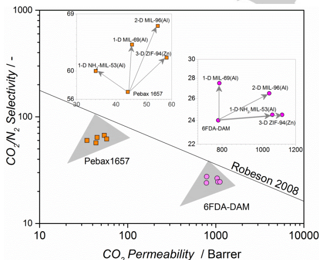
Figure 11. Robeson plot of CO 2 / N 2 couple (CO 2 selectivity versus CO 2 permeability) of MOF-MMMs and neat 6FDA-DAM and Pebax membranes at 298 K and 2 bar absolute feed pressure (mixed gases). The insets are the enlarged views of the corresponding membrane performance. The Robeson upper bound (2008) is shown for reference. The MOF loading in all MMMs is 25 wt.%.
