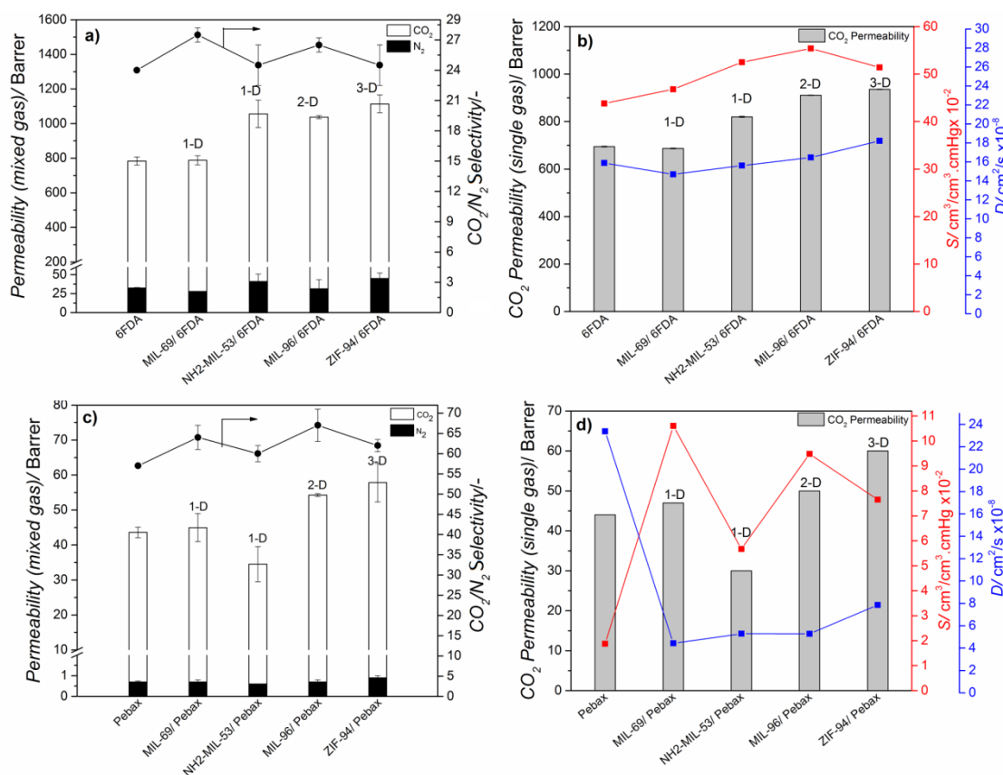
Figure 10. CO 2 /N 2 mixture permeability and selectivity of 6FDA-DAM (a) and Pebax (c) based membranes at 298 K and 2 bar absolute feed pressure (mixed gases). Single gas CO 2 permeability, solubility and diffusivity of 6FDA-DAM (b) and Pebax (d) based membranes at 295 K and 1 bar absolute feed pressure. Error bars correspond to standard deviation of duplicate membranes.
