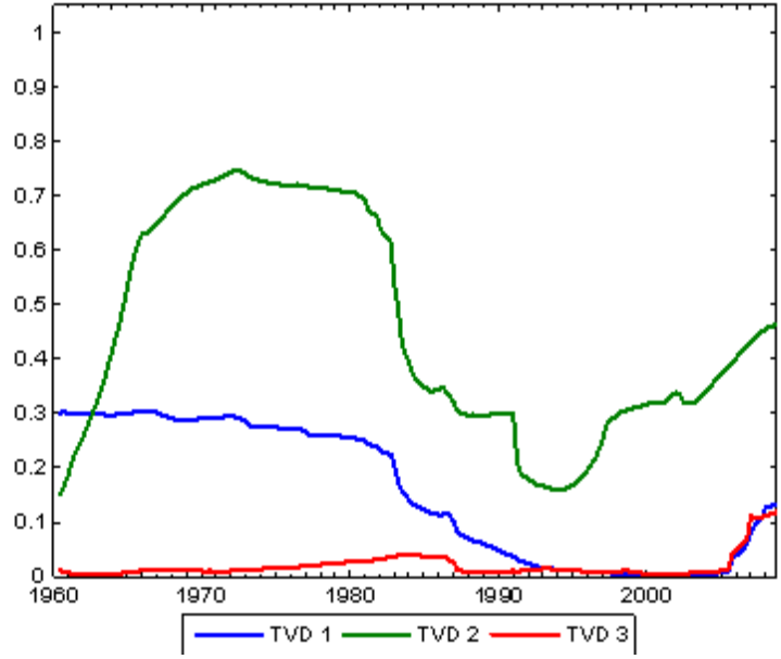
Figure 3: p(K_{3,t} = 1 | y) .
