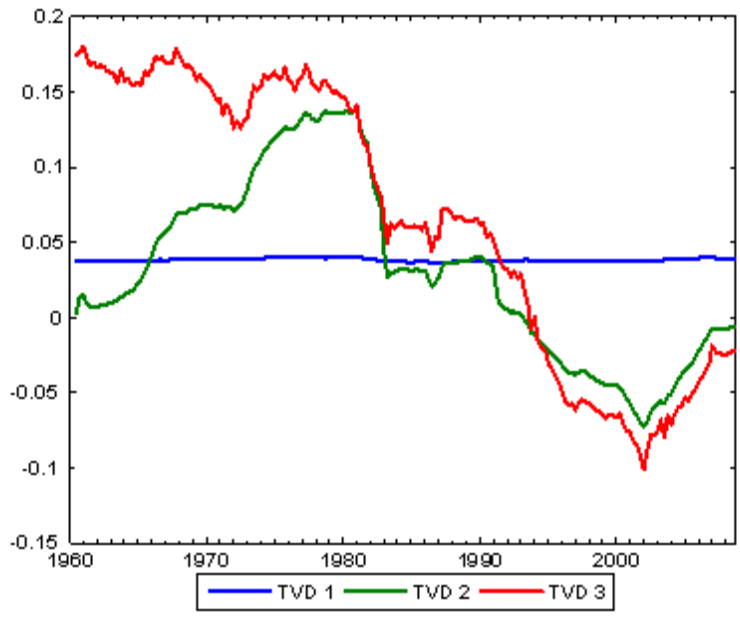
Figure 9: E(\gamma_{9,t}|y)
