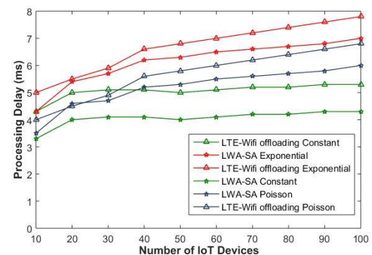
Fig. 12. Processing delay under different UE arrival rates.
