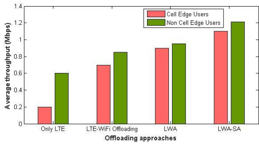
Fig 7. Throughput of UE in various offloading approaches.
