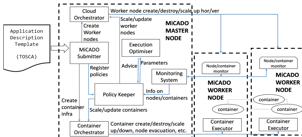
Figure 1. Generic architecture of MiCADO
