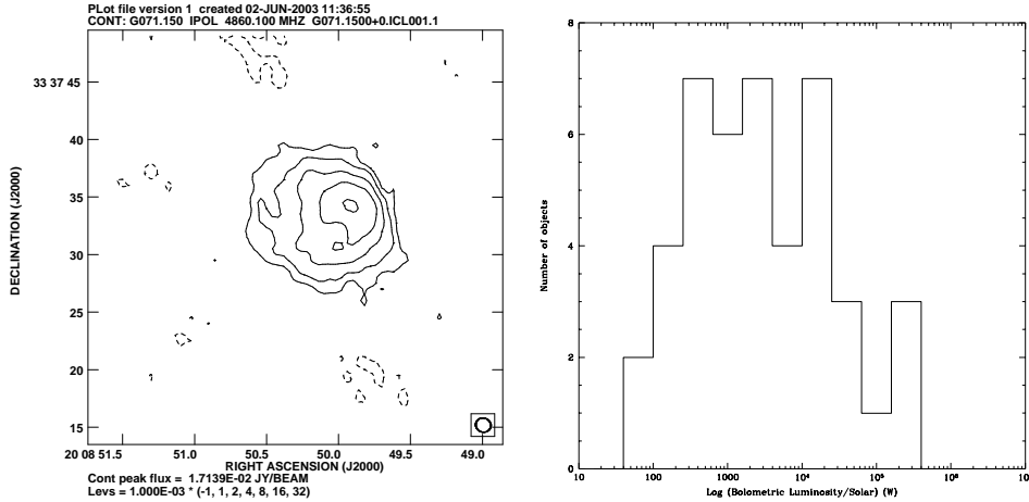
Figure 1. a) Example of a compact, cometary H II region found in the RMS sample. b) Luminosity distribution of a sample of outer galaxy RMS sources with good IRAS fluxes.
