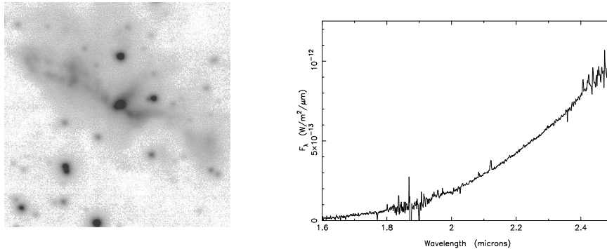
Figure 2. a) Near-IR K-band image of one strong MYSO candidate showing a probably bipolar nebula, extinction and associated cluster. b) Near-IR spectrum of the central source in a). Note the very red, feature-less continuum characteristic of MYSOs. The 2.12\mu\text{m} \text{H}_2 line is visible and this and other shock excited lines are strong along the length of the outflow. The range 1.80\mu\text{m} < \lambda < 1.95\mu\text{m} and \lambda > 2.39\mu\text{m} are affected by noise due to the atmosphere.
