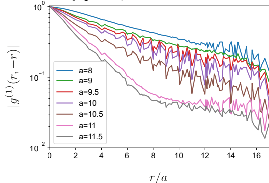
FIG. 9. Average first order correlation function g^{(1)}(r/a) vs. length r for various lattice constants of a 15 \times 15 condensate lattice.
