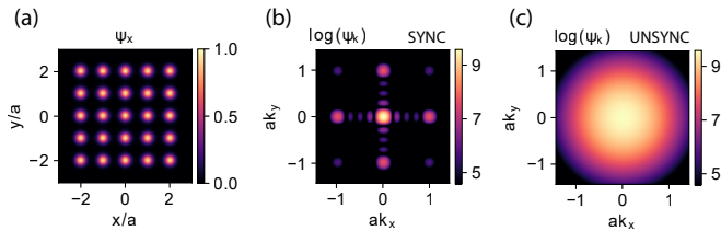
FIG. 7. Intensity of the synchronized phase in real (a) and reciprocal (b) space. (c) Intensity of the UNSYNC phase in momentum space. The only parameter is L/a = 0.22 .
