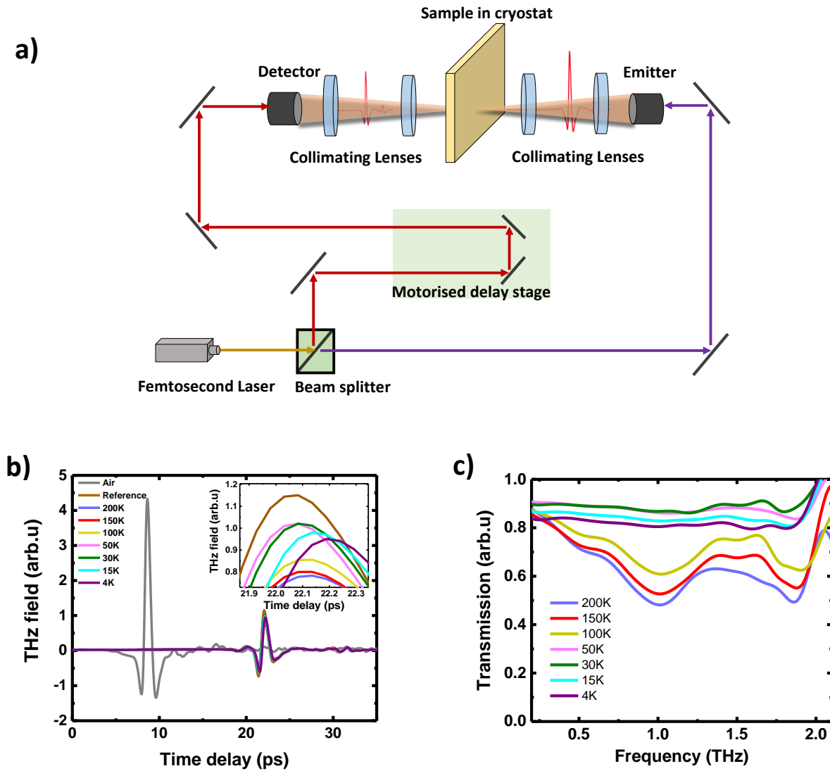
Figure 1. (a) Schematic of a THz-TDS optical setup. The light of a 60-mW pump laser of 90 fs duration, centered at 1560 nm, was split into two paths for THz generation (purple) and detection (red). (b) Time domain picosecond (ps) pulse response transmitted through air and a \text{Bi}_2\text{Se}_3 film of 23 QL (quintuple layer) at different temperatures. The inset shows a magnified pulse response transmitted through the \text{Bi}_2\text{Se}_3 film. The reference is transmission through (0001)-oriented sapphire substrate shown for 200 K. All the temperature measurements were performed in a cryostat with optical access with a base temperature of 4 K. (c) Normalized transmission amplitude spectra with respect to substrate at same temperature obtained from the Fourier transform of the temporal THz signal through \text{Bi}_2\text{Se}_3 from 4 K to 200 K.
