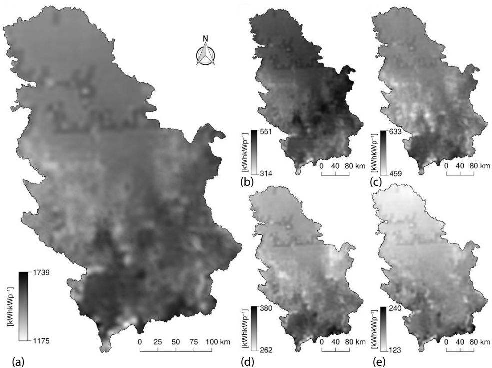
Figure 2. Electricity generation from a 1 kWp PV system; (a) the average annual values, (b) the average spring values, (c) the average summer values, (d) the average autumn values, (e) the average winter values
