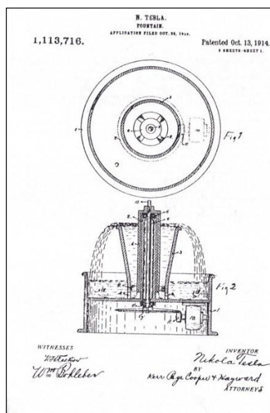
Fig. 1. Original Tesla's Fountain patent.
