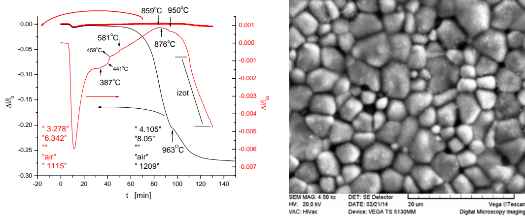
Fig. 1. Dilatograms of \text{ZnTiO}_3 sample sintered at 1200^\circ\text{C} and reheated at 1100^\circ\text{C} in the second run, with characteristic values and temperature intervals.
