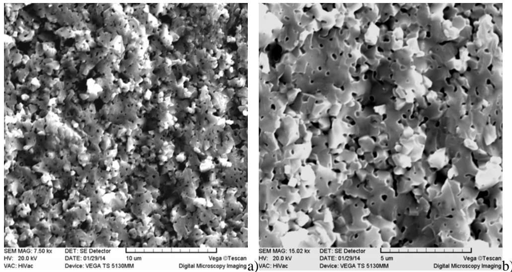
Fig. 9. ZnTiO 3 reheated 1100°C, 20 minutes, nitrogen atmosphere, a) 15 kx b)30 kx enlargement.
