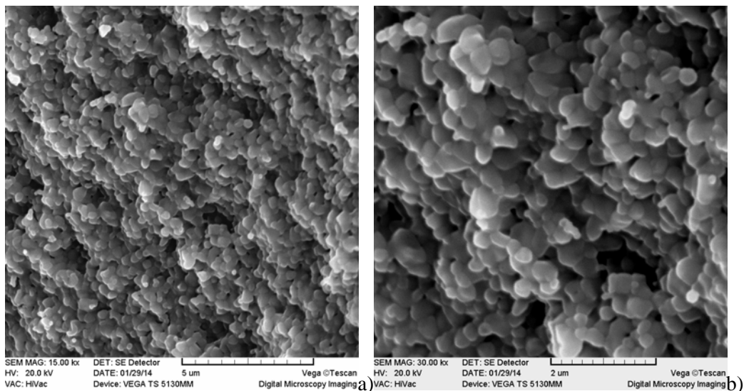
Fig. 7. ZnTiO 3 sintered 1100°C, 1h, a) 15 kx b) 30 kx enlargement.
