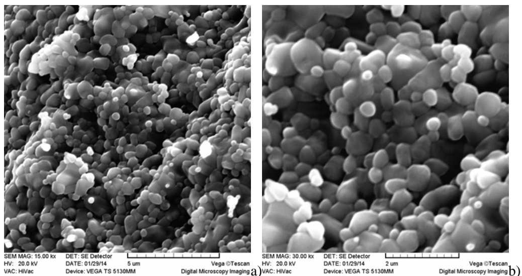
Fig. 8. ZnTiO 3 reheated 1100°C, 20 minutes, air atmosphere a) 15 kx b) 30 kx enlargement.
