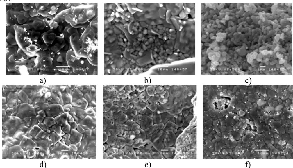
Fig. 3. SEM micrographs of \text{Ho}_2\text{O}_3 doped \text{BaTiO}_3 sintered at 1320^\circ\text{C} with a) 0.01wt% \text{Ho}_2\text{O}_3 , b) 0.1wt% \text{Ho}_2\text{O}_3 , c) 1wt% \text{Ho}_2\text{O}_3 and sintered at 1380^\circ\text{C} with d) 0.01wt% \text{Ho}_2\text{O}_3 , e) 0.1wt% \text{Ho}_2\text{O}_3 , f) 1wt% \text{Ho}_2\text{O}_3 .
