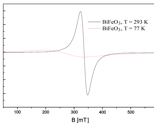
Figure 9. EPR spectra of the BFO powder measured at T = 293\text{ K} and T = 77\text{ K}
