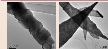
TEM (Y_{0.75}Gd_{0.25})_2O_3 600 polycrystalline rods
