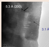
TEM (Y_{0.75}Gd_{0.25})_2O_3 600 polycrystalline rods
