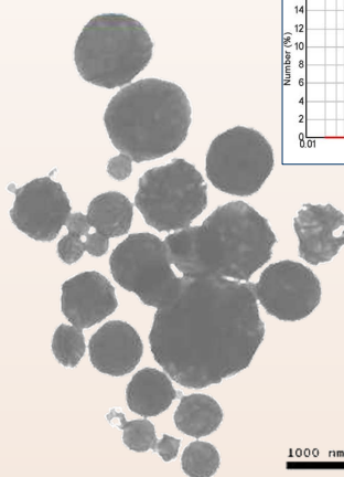
Microstructural characteristics of HT produced powders (Topas Academic)
