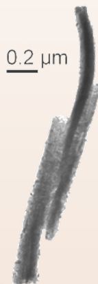
TEM (Y_{0.75}Gd_{0.25})_2O_3 600 polycrystalline rods
