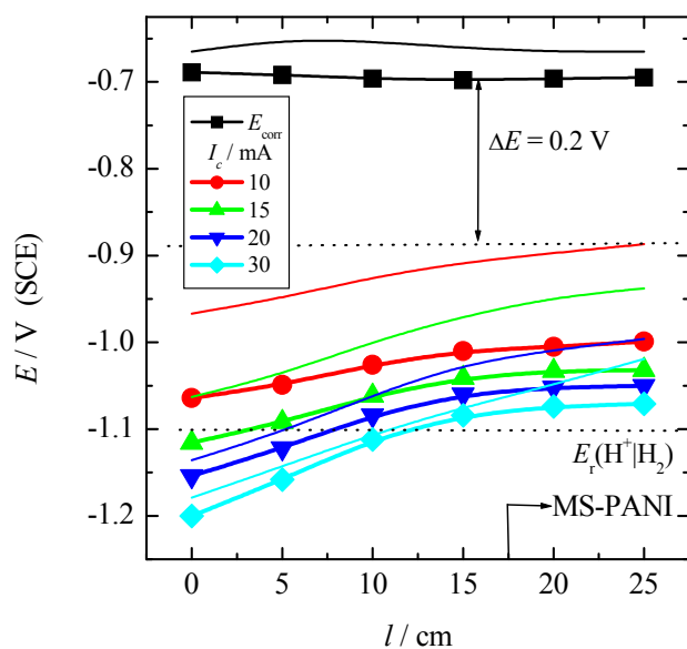
Figure 8. Dependence of the potential along the mild steel electrode partially covered with PANI for different currents in 3% NaCl solution; the lines represents the data from Fig 7.
