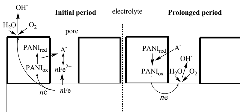
Figure 15. Proposed mechanism of the mild steel corrosion protection with PANI coatings.
