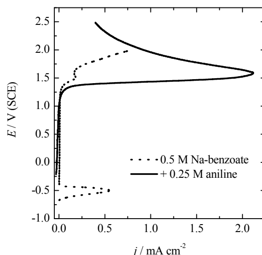
Figure 2. Anodic polarization curves ( v = 1 mV s ^{-1} ) of mild steel in a 0.5 M sodium benzoate solution and with an addition of 0.25 M aniline monomer.
