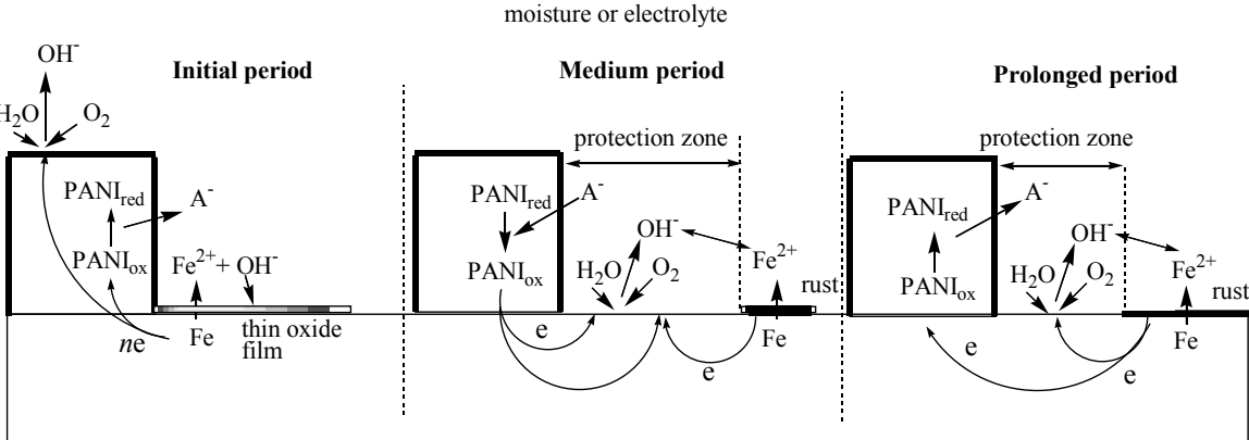
Figure 17. Proposed mechanism of the mild steel corrosion protection using a partial PANI coating.
