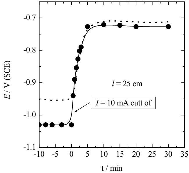
Figure 10. Dependence of the potential at l = 25 cm after the current was interrupted for mild steel (----) and mild steel partially covered with polyaniline (-●-).
