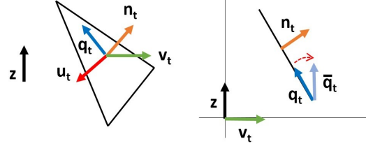
Fig. 5. Left: 3D view of the triangle with normal n_t , tangent frame u_t, q_t . Right: Side view of the z, v_t plane, showing the rotation of q_t around u_t .
