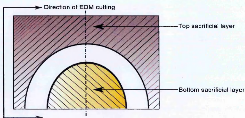
Figure 3.65. Schematic representation of the sacrificial layers attached on the Eshete mock-up for determination of 2D stresses along axial direction at the WCL.
