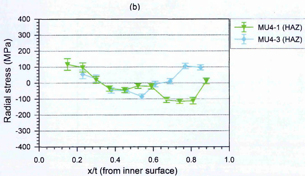
Figure 3.48. Radial stress distributions in the low heat input (MU4-1) and high heat input (MU4-3) pipes measured at the (a) the WCL and (b) the HAZ.
