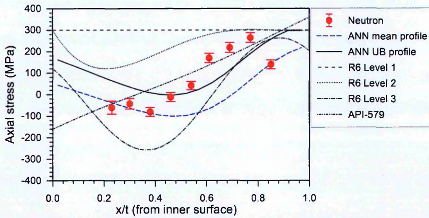
Figure 5.10. Comparison of upper bound profiles in the heat affected zone for the high heat input girth weld MU4-3 in the axial direction.
