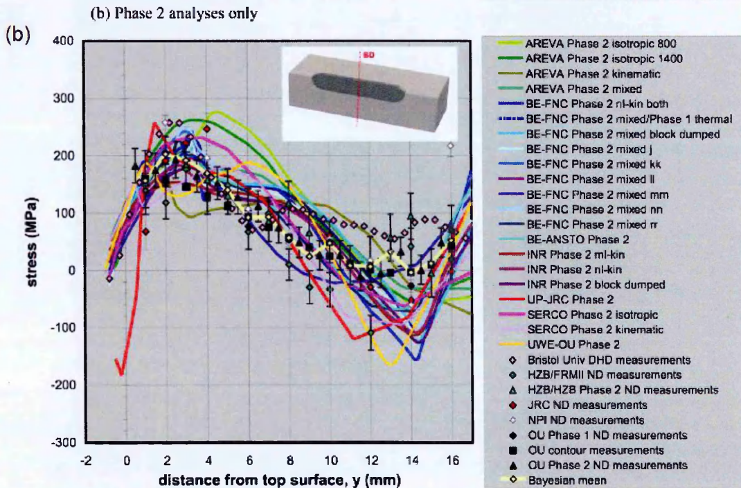
Figure 2.9. Comparison of measured and predicted (a) longitudinal stresses (b) transverse stresses along line BD through the plate thickness, and mid-width and mid-length in the weld bead of NeT- TG1 specimen; plate dimensions 120 mm × 80 mm × 17 mm with a weld length of 60 mm [91].
