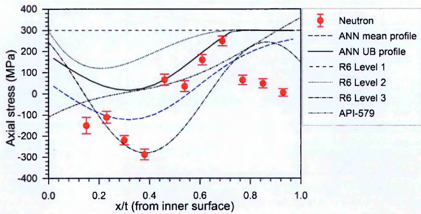
Figure 5.4. Comparison of upper bound profiles in the weld centre line for the high heat input girth weld MU4-3 in the axial direction.
