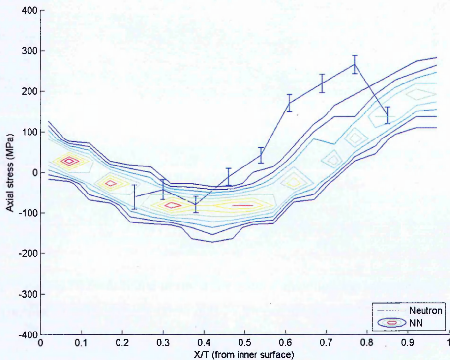
Figure 4.16. ANN model prediction of axial stress distribution of the STYLE pipe butt weld MU4-3 at the HAZ (Input parameters R/t = 4.5 , t = 25 mm and Q = 1.5 kJ/mm).
