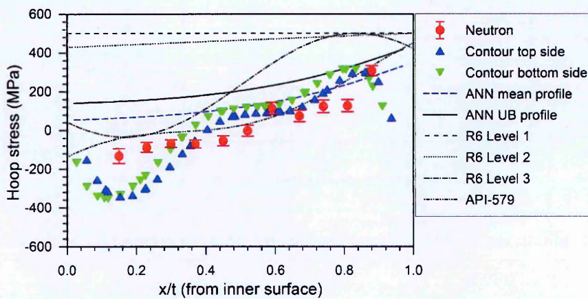
Figure 5.9. Comparison of upper bound profiles in the heat affected zone for the low heat input girth weld MU4-1 in the hoop direction.
