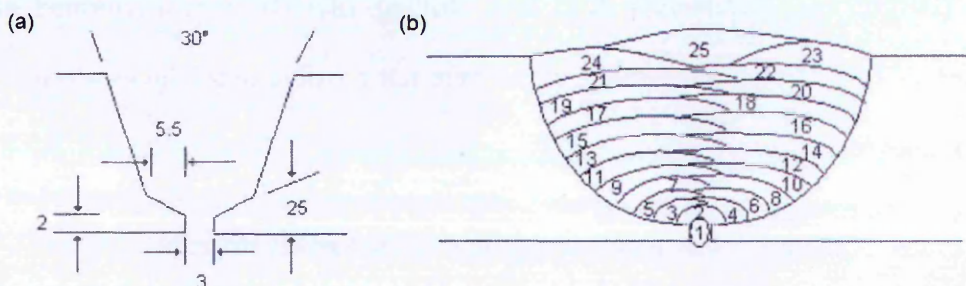
Figure. 3.58. (a) Weld groove preparation (b) Schematic showing weld pass sequence in the Eshshete 1250 pipe.
