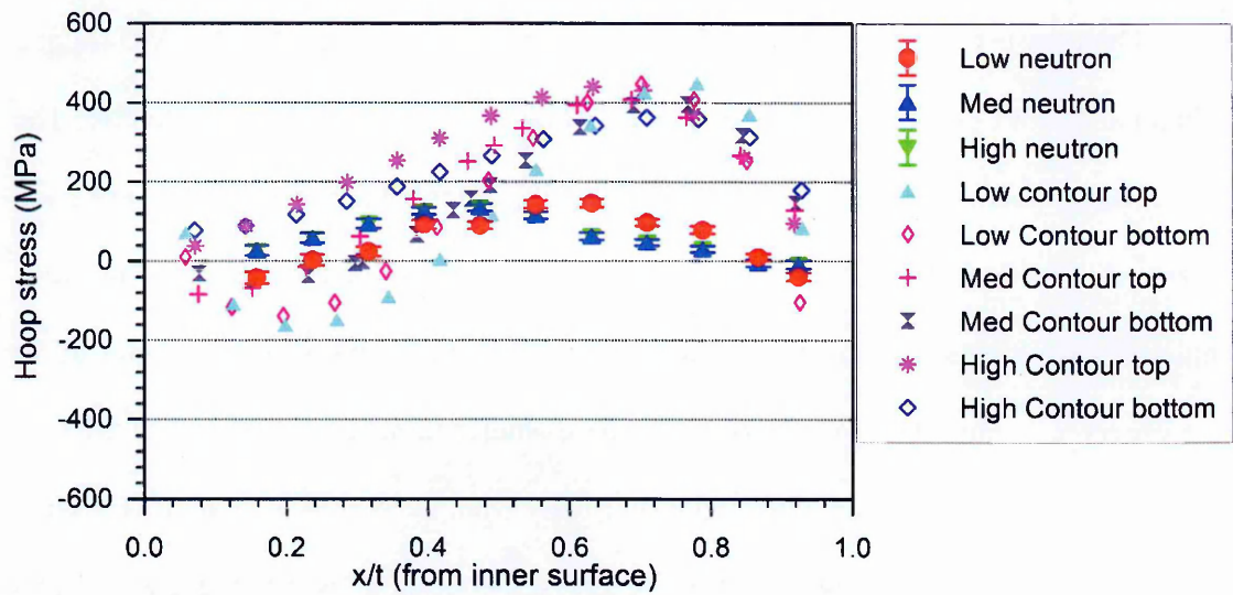
Figure 3.70. Comparison of hoop residual stress distributions at the WCL measured using neutron diffraction and the contour method in the thin pipes (Low, Med and high).
