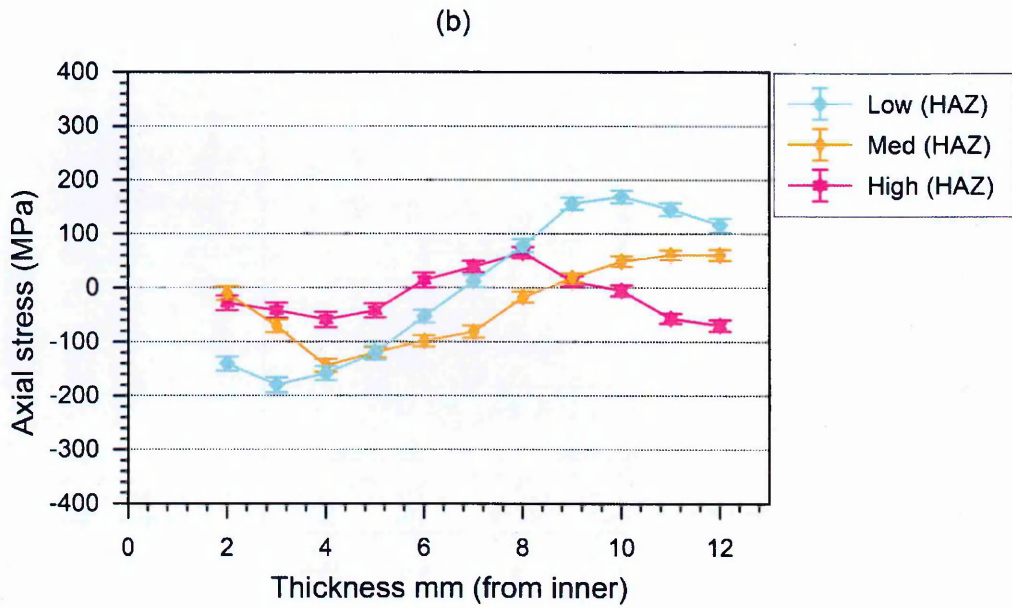
Figure 3.20. Axial stress distributions based on assumed plane stress conditions in the low, medium and high heat input pipes measured at (a) the WCL and (b) the HAZ.
