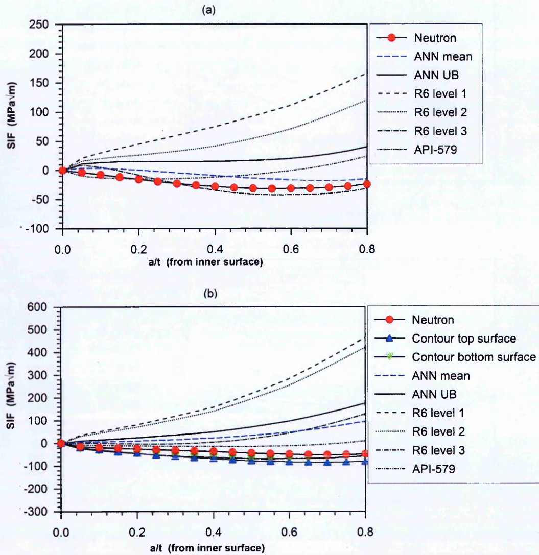
Figure 5.16. Comparison of SIFs at the heat affected zone of low heat input weld MU4-1 based on measurements and upper bound profiles for: internal surface breaking (a) circumferential crack (b) axial crack.
