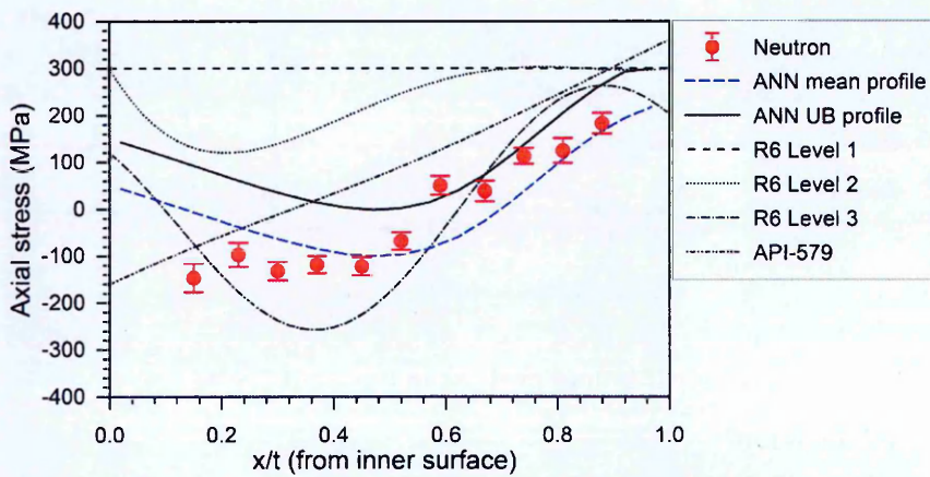
Figure 5.8. Comparison of upper bound profiles in the heat affected zone for the low heat input girth weld MU4-1 in the axial direction.
