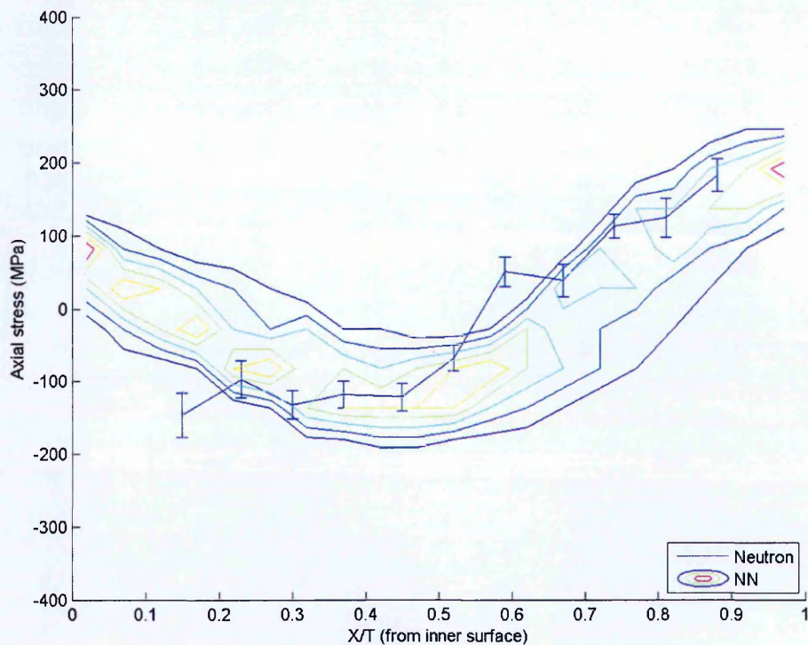
Figure 4.14. ANN model prediction of the axial stress distribution in the STYLE pipe butt weld MU4-1 at the HAZ (Input parameters R/t = 4.5 , t = 25 mm and Q = 0.8 kJ/mm).
