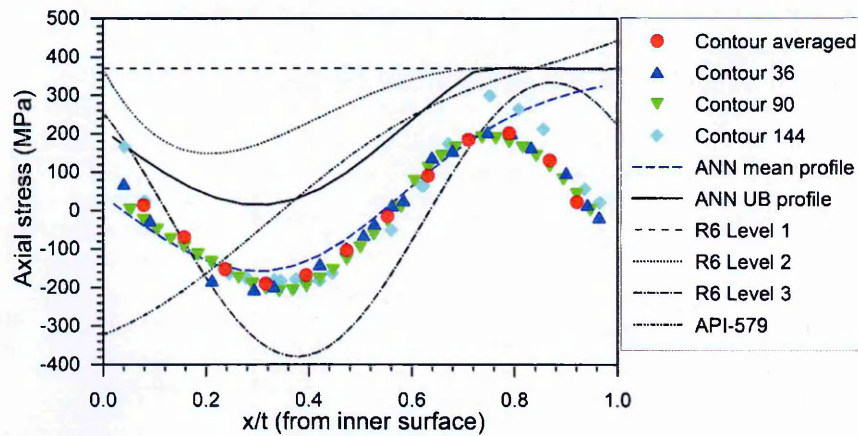
Figure 5.6. Comparison of upper bound profiles in the weld centre line of the Esshete girth weld in the axial direction.
