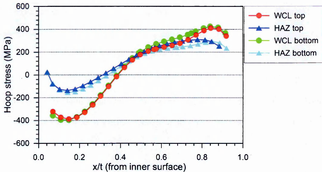
Figure 3.52. Hoop stress distributions at the WCL and HAZ measured contour method in the high heat input pipe (MU4-3).
