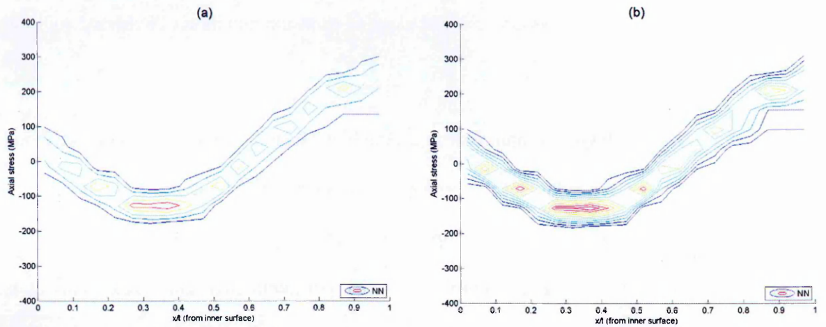
Figure 4.7. A comparison of the ANN predicted stress profiles using (a) raw data and (b) reduced data using interpolation tool for a low heat input pipe girth weld (MU4-1).
