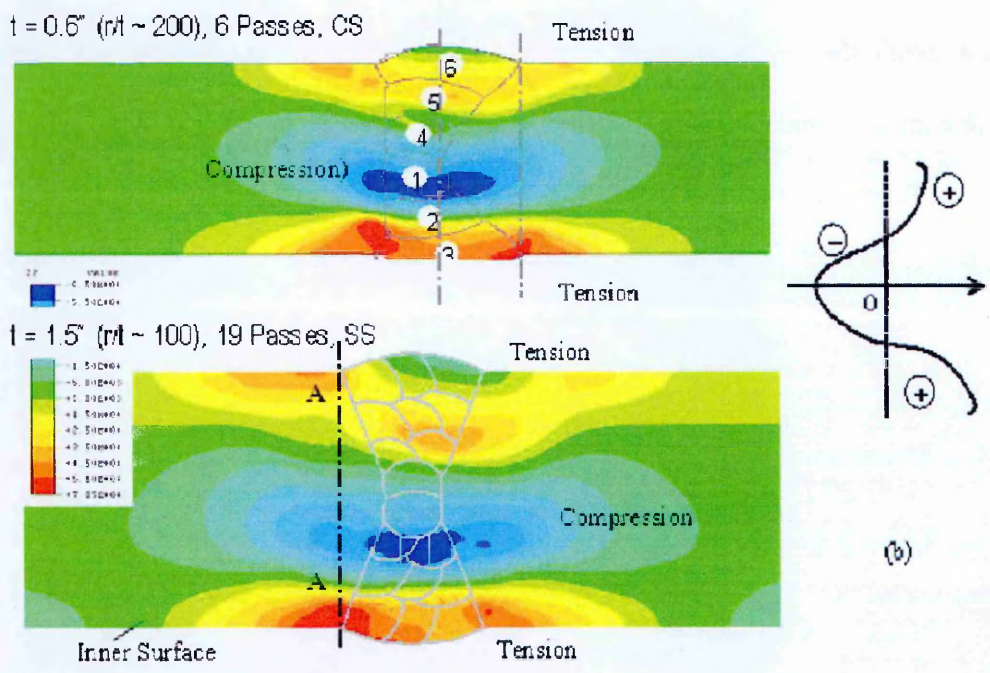
Figure 2.13. Two types of axial residual stress distributions in girth welds (a) “bending type” (b) “self-equilibrating” type [111].
