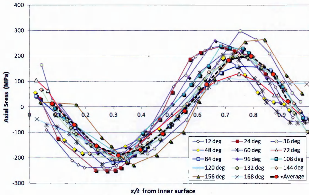
Figure 3.68. Comparison of axial stress profiles at various locations (12 deg., 24 deg., 36 deg..... 168 deg. and averaged stress profile across 45 deg across both sides of YY) at the WCL of the Eshete pipe.
