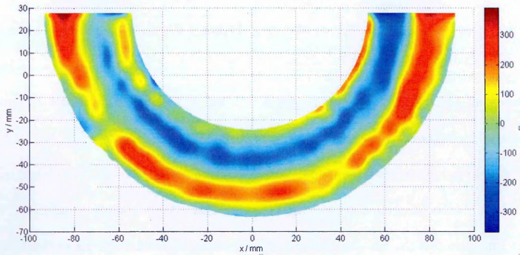
Figure 3.66. Cross-sectional view on a diametral-hoop plane of a 3D finite element model of the Eshete pipe girth weld ( R/t = 2.1 , t = 35 mm, heat input = 1.8 KJ/mm) showing a contour map of inferred axial residual stresses at the weld centre-line on the pipe wall cut surfaces that have been relieved during a contour residual stress measurement.
