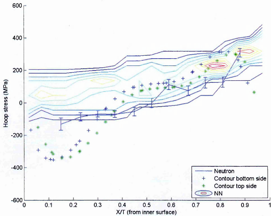
Figure 4.15. ANN model prediction of hoop stress distribution of the STYLE pipe butt weld MU4-1 at the HAZ (Input parameters R/t = 4.5 , t = 25 mm and Q = 0.8 kJ/mm).
