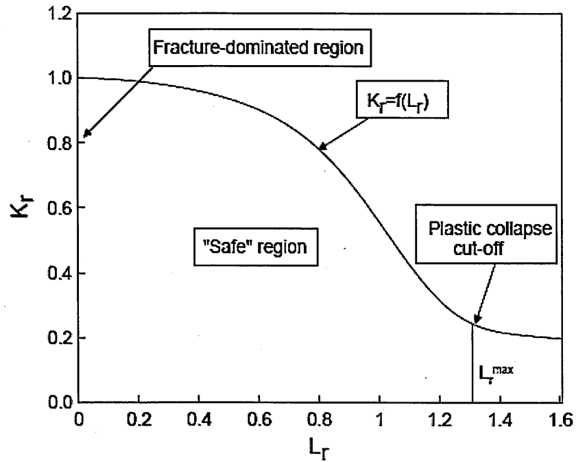
Figure. 2.12. Assessment curve of the R6 FAD [4]
