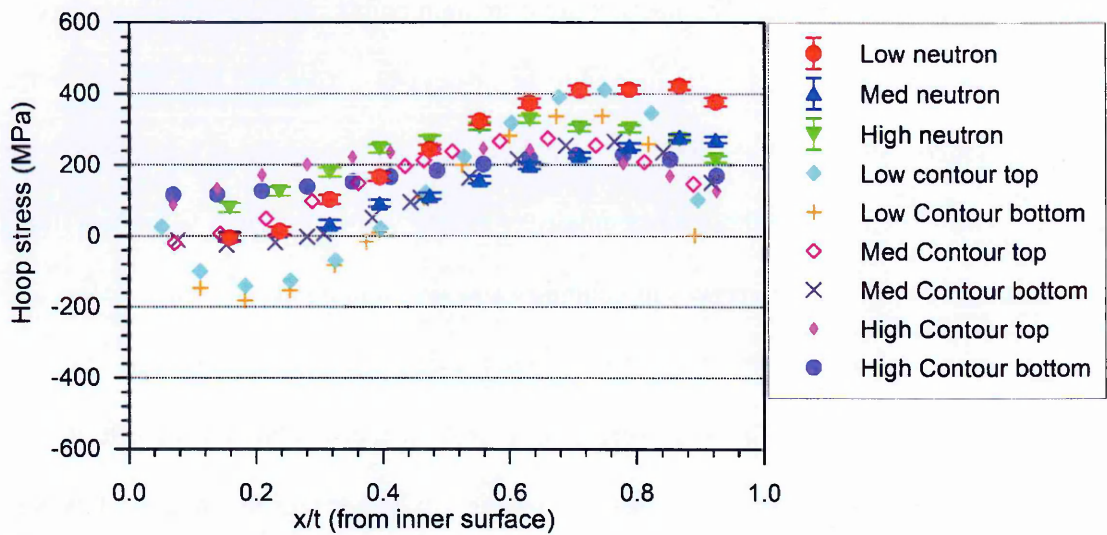
Figure 3.71. Comparison of hoop residual stress distributions at the HAZ measured using neutron diffraction and the contour method in the thin pipes (Low, Med and high).
