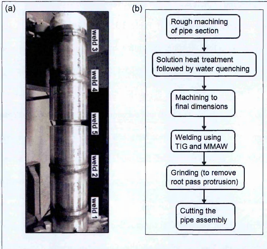
Figure 3.57. (a) Photograph of the Eshshete 1250 pipe assembly containing series of girth welds (b) Manufacturing history of the welded Eshshete pipe weldments [17, 18].
