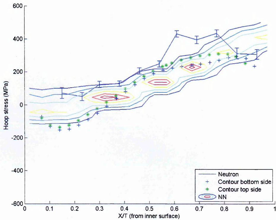
Figure 4.17. ANN model prediction of hoop stress distribution of the STYLE pipe butt weld MU4-3 at the HAZ (Input parameters R/t = 4.5 , t = 25 mm and Q = 1.5 kJ/mm).
