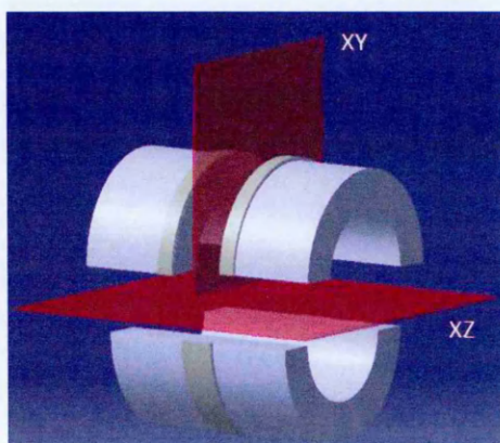
Figure 3.64 Schematic illustration of the location and plane of the performed contour cut for the measurement of axial stresses at the weld centre line in the Eshete weld.
