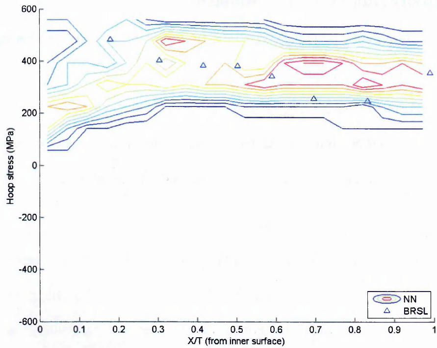
Figure 4.22. Sensitivity studies on the effect of R/t in the model distribution of hoop stress distribution of the Hypothetical pipe weld (H3) at the WCL (Input parameters R/t = 25 , t = 40 mm and Q = 1.85 kJ/mm).
