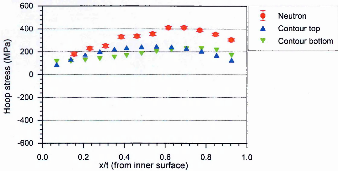
Figure 3.36. Comparison of hoop residual stress distributions at the HAZ measured using neutron diffraction and the contour method in the high heat input pipe (High).
