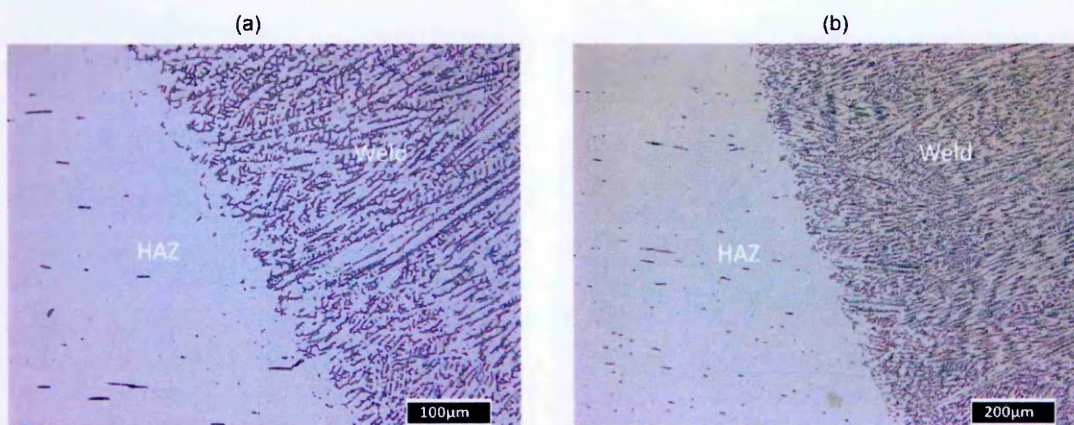
Figure 3.42. Microstructural analysis at the fusion boundary of (a) low heat input MU4-1 b) high heat input MU4-3 pipe components.
