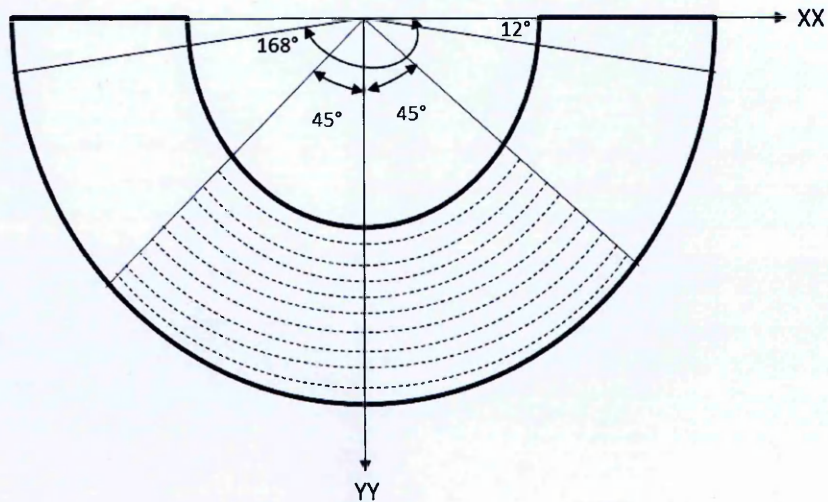
Figure 3.67. Schematic illustration of the location of through-thickness stress profiles in the Eshete weld.
