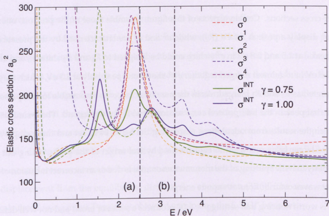
Figure 5.12: Partial wave analysis of the MS cross section of (\text{HCOOH})_2 , with input T -matrices generated using the 6-31G basis set, a = a_c = 8 a_0 . Cutoff and interpolated cross sections are shown; vertical lines mark the cutoff energy E^3 when (a) \gamma = 1.00 and (b) \gamma = 0.75 .
