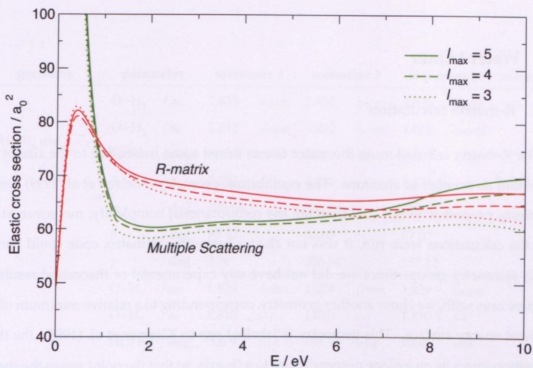
Figure 4.16: R -matrix and Multiple Scattering elastic cross sections for the Z_2 dimer geometry, where a different number of partial waves was included. The contribution of higher partial waves has a similar effect on both calculations; therefore it does not improve the comparison.
