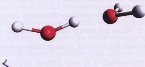
Figure 6.3: Ball-and-stick model of (\text{H}_2\text{O})_2 , equilibrium geometry. The monomer on the left is the bond donor, in plane, while the other is the bond acceptor, out of plane.
