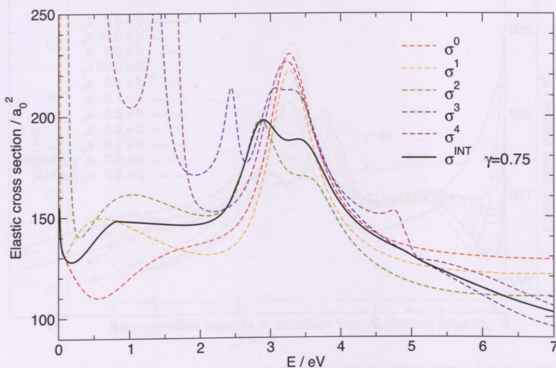
Figure 5.14: MS cutoff and interpolated cross sections when the HCOOH—HCOOH distance is increased by 1 a_0 from the equilibrium one ( R_{1,2} = 6.698 a_0 ).
