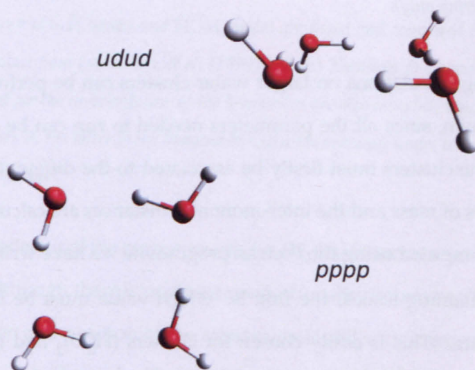
Figure 4.24: Ball-and-stick models of (\text{H}_2\text{O})_4 , udud and pppp geometries.
