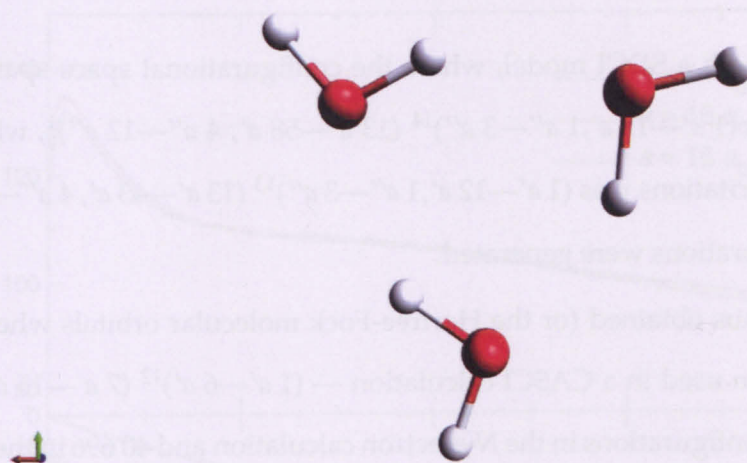
Figure 4.17: Ball-and-stick models of (\text{H}_2\text{O})_3 , ppp geometry.
