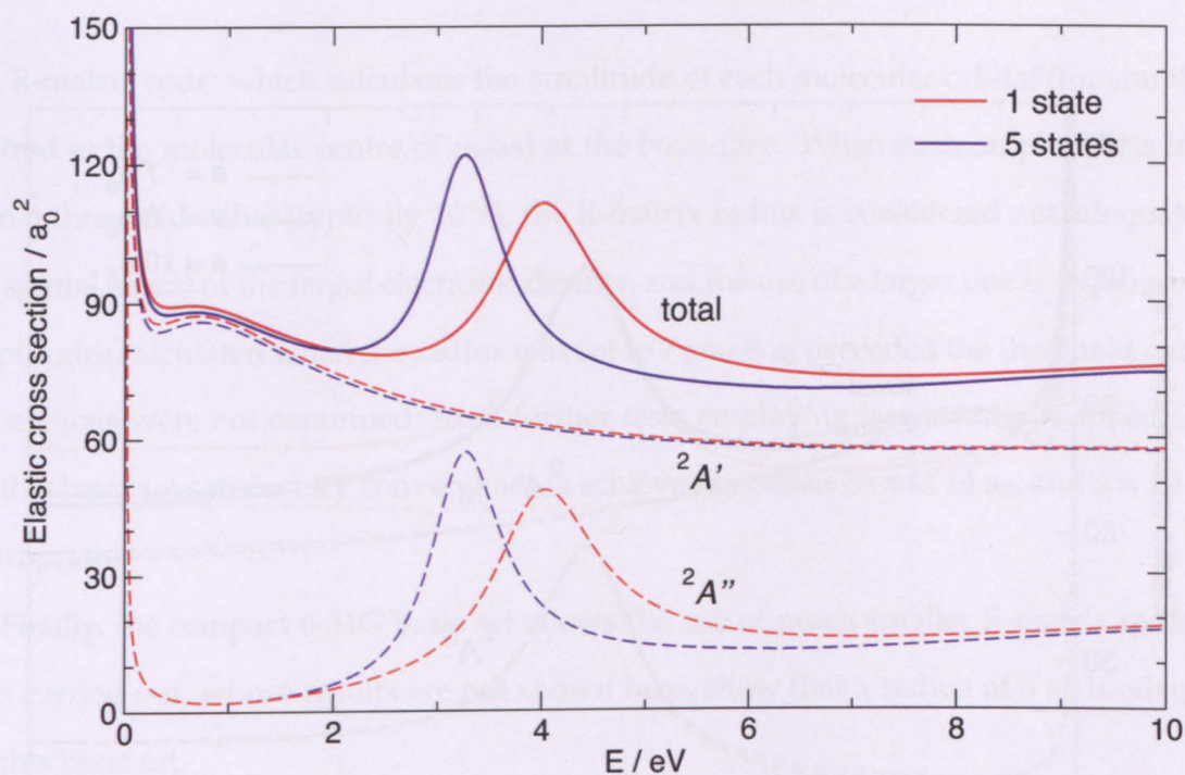
Figure 5.3: Elastic cross sections for the R-matrix calculations performed using the same basis set (6-31G**) and R-matrix radius ( a = 10 a_0 ), but different number of states; HF-SCF orbitals were employed.
