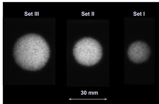
Figure 4. UV fluorescence images of wet areas taken after \approx 45000 min of spreading into a sand bed prepared using R \approx 0.26 mm particles. From left to right the images are from runs III, II and I, as seen in Tables I and II.
