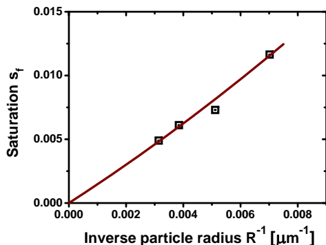
Figure 12. Saturation s_f as a function of R^{-1} shown by symbols. The solid line is the fit s_f = A_f R^{-1} + B_f R^{-2} at A_f = 1.5 \mu\text{m} and B_f = 29 \mu\text{m}^2 .
