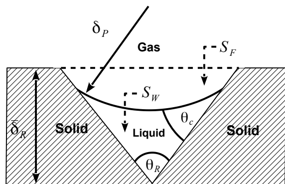
Figure 9. Illustration of the model groove geometry with an opening angle \theta_R and a contact angle \theta_c used in the analysis of \kappa_0 and s_0 . In the illustration, the groove is not fully filled in. The liquid filament cross-section area S_W is shown with the free surface at the capillary pressure p = -\gamma/\delta_P . A fully filled-in groove at a different pressure is illustrated by the pinned interface shown by a dashed line, surface area S_F .
