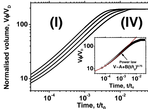
Figure 14. Simulation of spreading in a three-dimensional spherically symmetric case using augmented superfast diffusion model (54) with initial distribution (57) at \lambda_a = 0.3 , s_a = 0.4 , \alpha_g = 16.5 , \beta_g = 1.65 , f_0 = 1 and s_f = 0.0052 , but at different values of parameter s_f - s_0^e . Normalised wet volume V\phi/V_D (inverse average saturation \bar{s}^{-1} , solid lines) as a function of the reduced time t/t_0 , t_0 = L_0^2/D_0^e . From left to right: (I) s_f - s_0^e = 0.0001 , (II) s_f - s_0^e = 0.0002 , (III) s_f - s_0^e = 0.0004 , (IV) s_f - s_0^e = 0.0008 . Inset shows the power law V\phi/V_D = A + B(t/t_0)^{0.75} (solid line, brown) in comparison with the numerical data (symbols, black) at s_f - s_0^e = 0.0008 .
