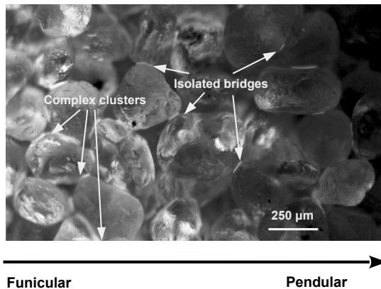
Figure 3. An UV fluorescence image of the liquid (TEHP) distribution in sands in the transition from the pendular to the funicular regimes of wetting, at s > 10\% .
