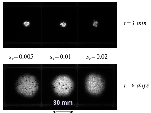
Figure 19. Spreading of TEHP liquid drops ( V_D = 6 \text{ mm}^3 ) in pre-wetted sands with different background saturations levels s_r = 0.5, 1 and 2\% . UV fluorescence wet spot areas taken at t = 3 \text{ min} and at t = 6 \text{ days} after the deposition of the drops on the sand bed.
