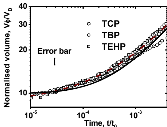
Figure 7. Spreading TCP, TEHP and TBP liquid drops ( V_D = 3 mm 3 ) in sands with R = 0.25 mm in one-dimensional geometry, as in Fig. 6. Comparison between experimental data and simulations using superfast diffusion model model (54) with initial distribution of saturation given by (60). Normalised wet volume V\phi/V_D (inverse average saturation \bar{s}^{-1} ) as a function of the reduced time t/t_0 , where t_0 = L_0^2/D_f for experimental data and the numerical results were scaled by t_0 = L_0^2/D_0^e . Experimental data are shown by symbols and simulation is presented by the solid line. Parameters of the simulations and the fitting are summarized in Table II. The dashed line (brown) is the fit V\phi/V_D = A + B(t/t_0)^{0.5} at A \approx 8.5 and B \approx 340 .
