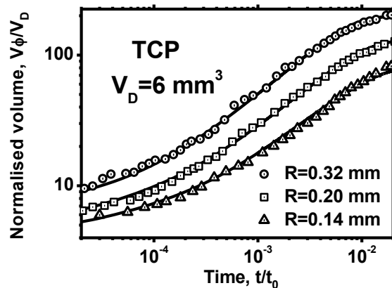
Figure 18. Spreading TCP liquid drops ( V_D = 6 \text{ mm}^3 ) in sands with different grain radii R = 0.14, 0.20 and 0.32 \text{ mm} . Comparison between experimental data and simulations using superfast diffusion model model (54) with initial distribution of saturation given by (57). Normalised wet volume V\phi/V_D (inverse average saturation \bar{s}^{-1} ) as a function of the reduced time t/t_0 , where t_0 = L_0^2/D_f for experimental data and the numerical results were scaled by t_0 = L_0^2/D_0^e . Experimental data are shown by symbols and simulations are presented by solid lines. Parameters of the simulations and the fitting are summarized in Table II.
