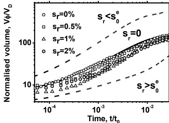
Figure 20. Spreading of TEHP liquid drops ( V_D = 6 \text{ mm}^3 ) in pre-wetted sands with different background saturations levels s_r = 0, 0.5, 1 and 2\% . Normalised wet volume V\phi/V_D (inverse average saturation \bar{s}^{-1} ) as a function of the reduced time t/t_0 , where t_0 = L_0^2/D_f for experimental data and the numerical results were scaled by t_0 = L_0^2/D_0^e . The experimental results are shown by symbols. The results of numerical simulations are shown by solid lines ( s_r = 0\% ) and by dashed lines s_r = 1\% and s_r = 0.5\% .
