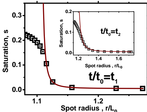
Figure 16. Simulation of spreading in a three-dimensional spherically symmetric case using augmented superfast diffusion model (54) with initial distributions given by (57) at \lambda_a = 0.2 and s_a = 0.5 . Saturation s(r, t) as a function of the reduced spot radius r/L_0 at fixed values of \alpha_g = 16.5 , \beta_g = 1.65 , f_0 = 1 , s_f = 0.0052 and s_f - s_0^e = 0.0002 . A comparison between the asymptotic solution (58) (solid line, brown) and the numerical solution at t = t_1 = 3 \times 10^{-6} shown by symbols, W_0 \approx 287 . The insert shows a similar comparison, but at t/t_0 = t_2 = 6 \times 10^{-5} , W_0 \approx 62 .
