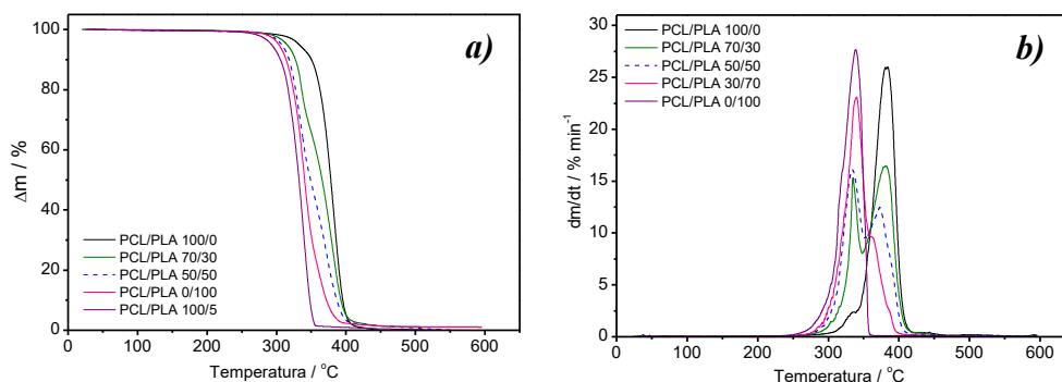
Slika 6. TG (a) i DTG (b) krivulje PCL/PLA mješavina Fig. 6. TG (a) and DTG (b) curves of PCL/PLA blends
