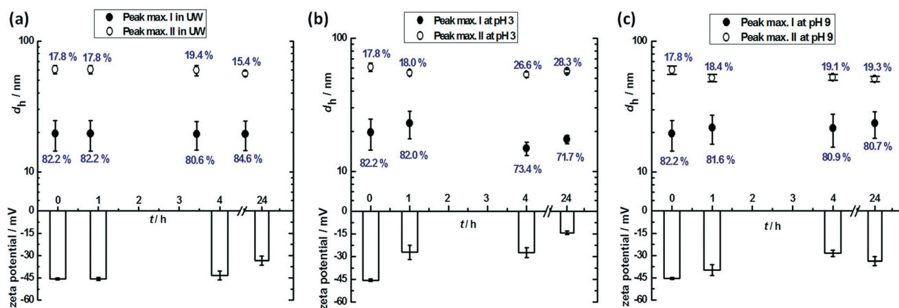
Fig. 3 Change in hydrodynamic diameter ( d_h ) and zeta potential of AgNPs in a) ultrapure water (UW), b) a medium with pH 3 and c) a medium with pH 9 during 24 hours at 25 °C. The mean volume % of particle populations with different sizes are indicated.
