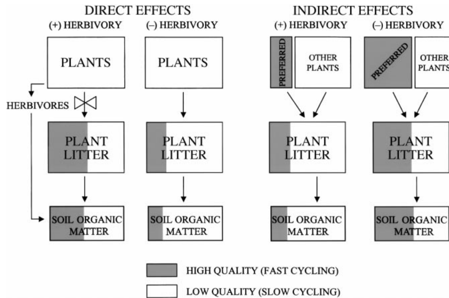
FIG. 1. Direct effects of herbivores tend to increase the proportion of the soil organic matter that is high quality (fast cycling) by increasing the quality of plant litter and by direct inputs of low C:N organic matter into the soil. Conversely, selective foraging may alter plant community composition such that the plant litter produced in the presence of herbivory is of lower quality (e.g., higher C:N ratio, more recalcitrant secondary chemicals) than that produced in the absence of herbivory.
