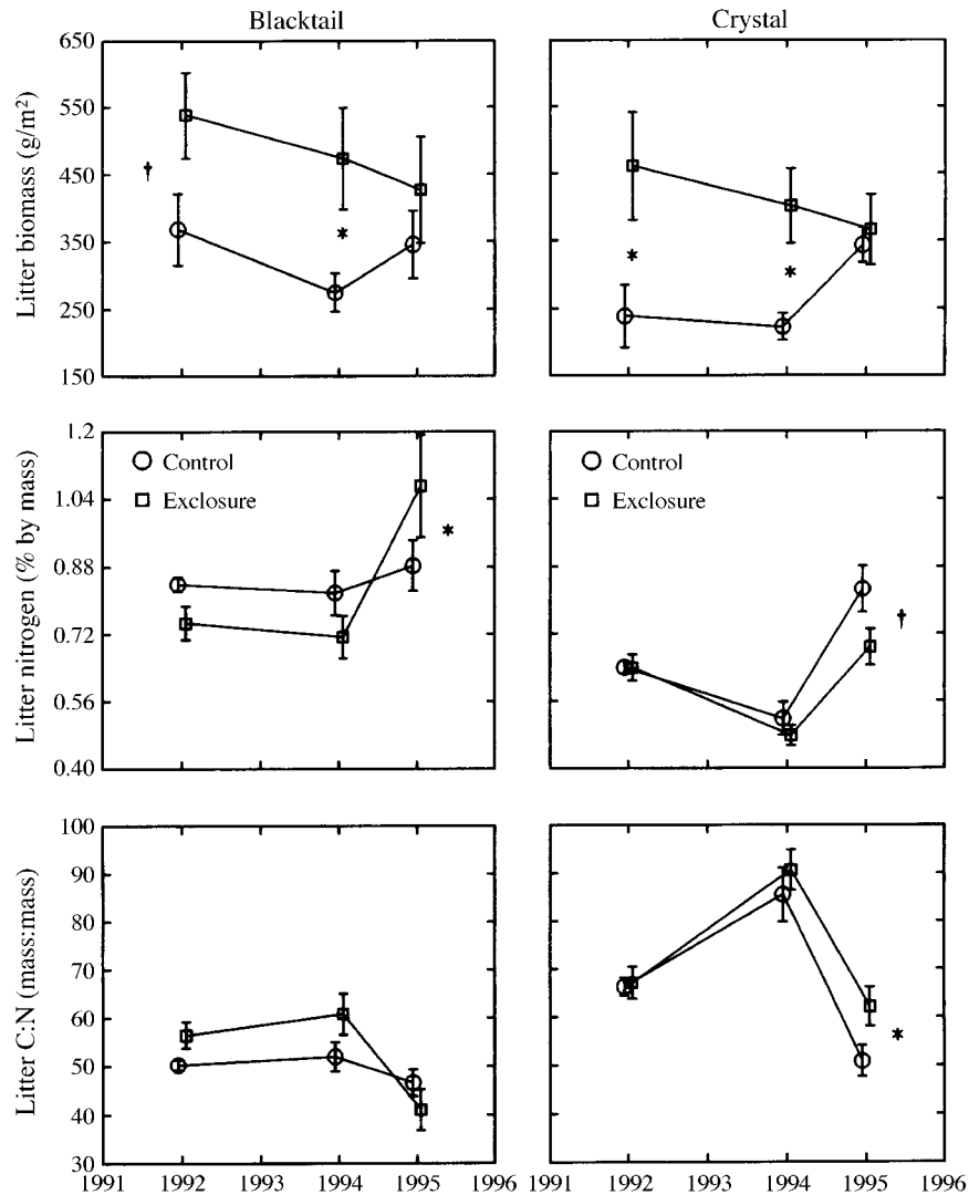
FIG. 3. Mean ( \pm 1 SE) biomass, nitrogen content, and C:N ratio of standing dead plant litter at the end of the growing season, after plant senescence. For Blacktail data, differences between experimental and control means within a year were tested using Tukey's hsd test (test statistic Q calculated with the error term from repeated-measures ANOVA). For Crystal data, because repeated-measures ANOVA could not be performed due to missing data, differences between means were tested using Bonferroni-adjusted individual ANOVAs on each year's data. For all treatments and years, n = 8 , except for Crystal 1992, where n = 6 .
