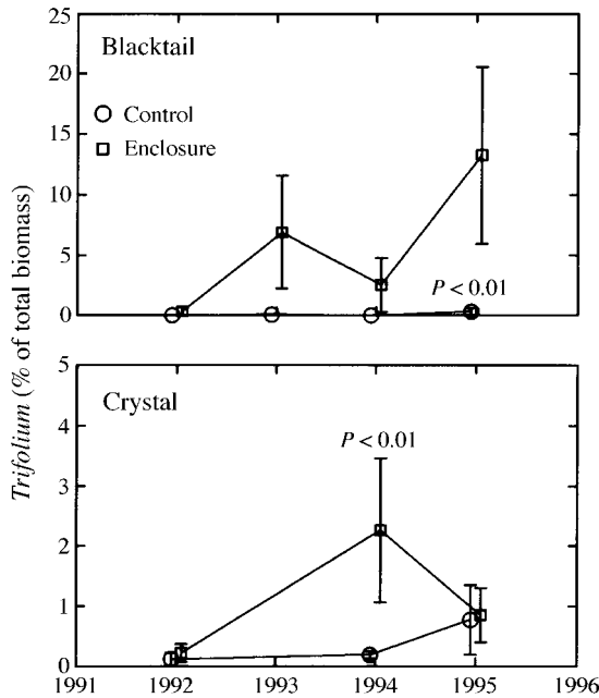
FIG. 4. Relative biomass (percentage of peak above-ground biomass) of Trifolium spp. at Blacktail and Crystal. P values are probabilities associated with Tukey's hsd test ( Q calculated with the error term from repeated-measures ANOVA) for treatment differences within each year's data. Only P values <0.10 are reported. Error bars represent \pm 1 SE; n = 8 for all years and treatments.
