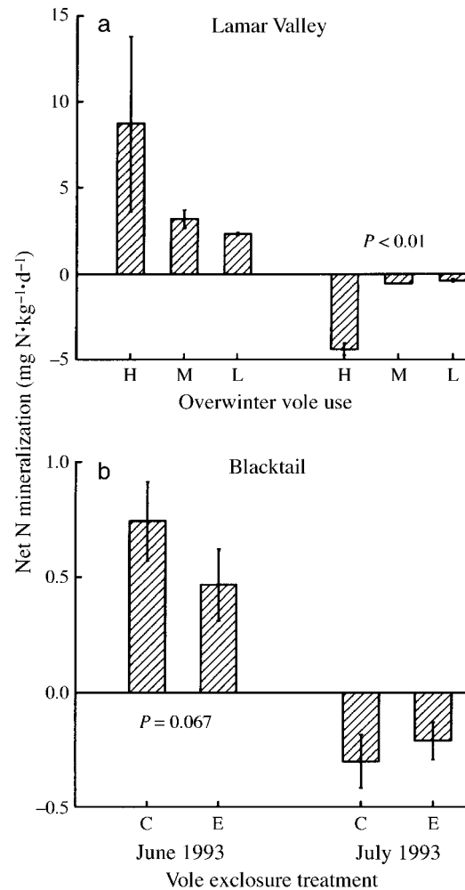
FIG. 6. Net nitrogen mineralization measured in the field during the growing season following a vole population peak at two riparian sites in northern Yellowstone Park. Methods are after Adams and Attiwill (1986) and Frank et al. (1994). (a) Month-long nitrogen mineralization ( \text{NO}_3^- + \text{NH}_4^+ ) during June and July 1993 at Lamar Valley (a riparian site in northern Yellowstone Park), on plots that experienced high (H), medium (M), and low (L) vole use over the 1992–1993 winter. (b) Month-long nitrogen mineralization in control plots (C) and exclosures (E) at Blacktail in 1993. P values are from one-way, blocked ANOVA. All probabilities less than 0.10 are shown; n = 3 at Lamar Valley, and n = 8 at Blacktail. Error bars are \pm 1 SE.
