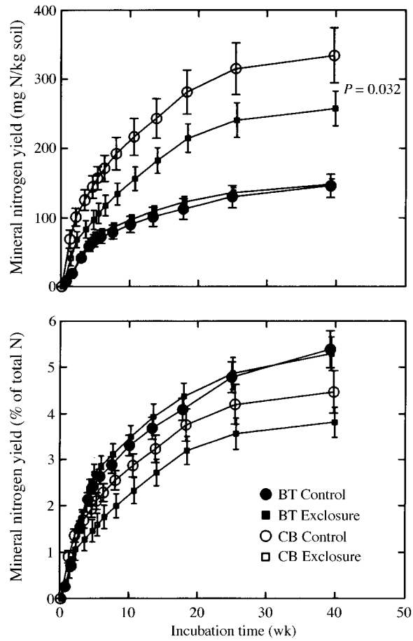
FIG. 5. Cumulative laboratory mineralization ( \text{NO}_3^- + \text{NH}_4^+ ) of soils collected in 1995 from Blacktail (BT) and Crystal (CB) controls and enclosures: top, absolute mineralization; bottom, mineralization as a percentage of total nitrogen in the soil. The P value is associated with the treatment effect of blocked ANOVA on cumulative nitrogen yield (Crystal) at the end of the experiment ( F = 8.87 ; df = 1, 5 ). Means for Crystal control plots exclude two outliers; otherwise, n = 8; error bars represent \pm 1 SE.
