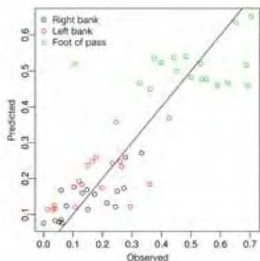
Model of the probability of recapture of marked glass eels released downstream and at the foot of a fish pass as a function of various individual and environmental criteria (size and condition of individuals, point of release, depth of water, temperature, cloud cover, day in lunar month, etc.).
