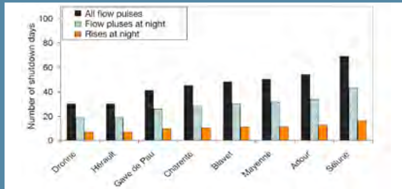
Figure 18. Potential turbine-shutdown durations for different managements scenarios in eight French rivers.
