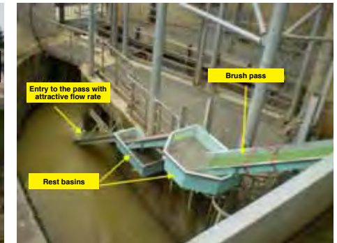
Eel pass at the Golfech dam (Garonne river). View of the lower section. © F. Travade, EDF
