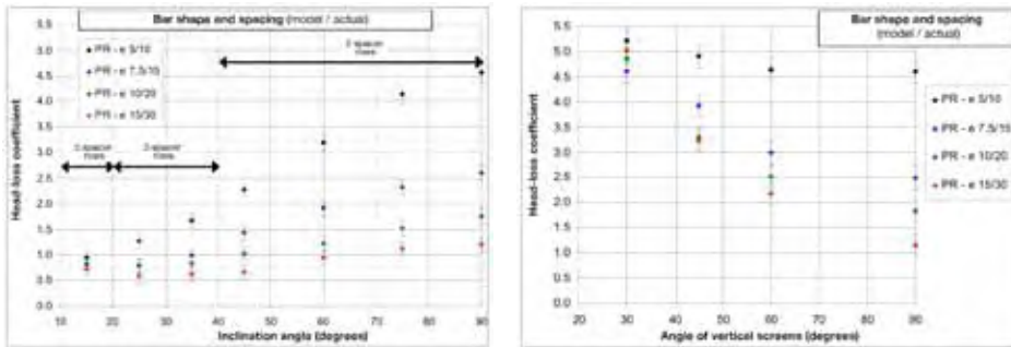
Head-loss coefficients as a function of the screen inclination angle or angle to the flow, and of the bar spacing (rectangular PR bars). The arrows indicate the number of submerged spacer rows between the bars.
