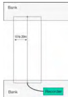
Layout of a Nedap station.
