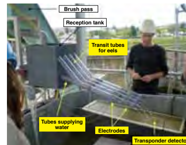
ELFES-ELTA electronic counter installed at the head of the Golfech fish pass for elvers. © L. Carry, MIGADO
