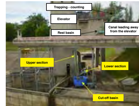
Eel pass at the Golfech dam (Garonne river). Overall view. © F. Travade, EDF
