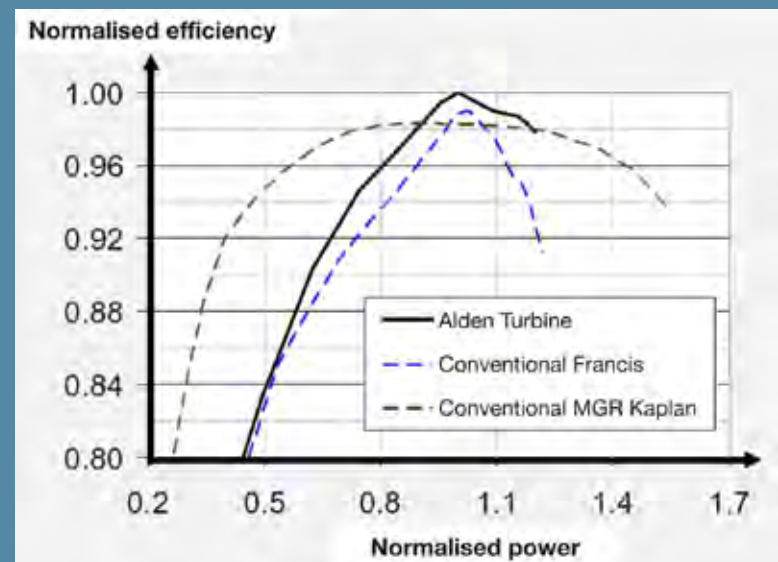
Figure 13. Comparative performance levels of Alden, Francis and Kaplan turbines.
