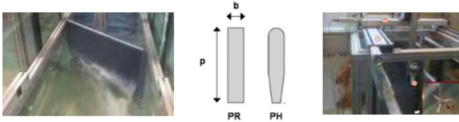
On the left, a screen angled 45°, seen from downstream, in the CEAT hydraulic channel. In the centre, the two bar shapes that were tested. On the right, the ADV 3D system with its automatic motion controller.
