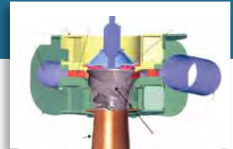
Alden fish-friendly turbine (cross-sectional view). © EPRI
