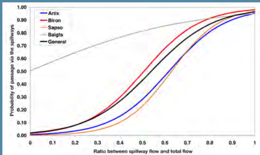
Figure 12. Model of the probability of passage via the spillway as a function of the ratio between the spillway flow and the total river flow.
