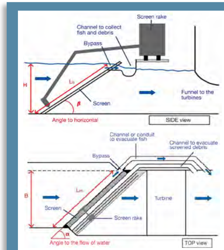
Figure 14. Simplified diagram of «fish friendly» water intakes, inclined (upper diagram) and angled (lower diagram). (Courret and Larinier, 2008)
