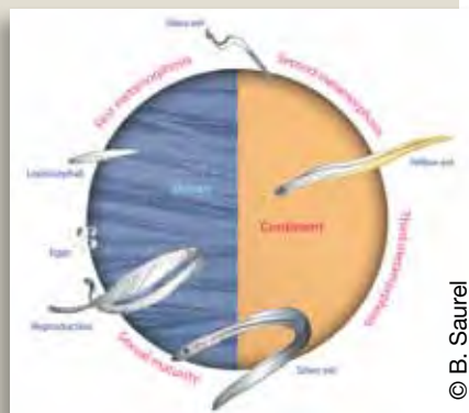
Life cycle of the European eel (source: Dekker, 2000).
