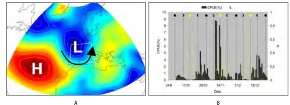
A. An example of weather. L and H are atmospheric low and high-pressure zones. The black arrow indicates the direction and the shape of the low-pressure weather front.
