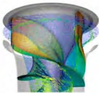
Digital modelling of the Alden turbine. © EPRI
