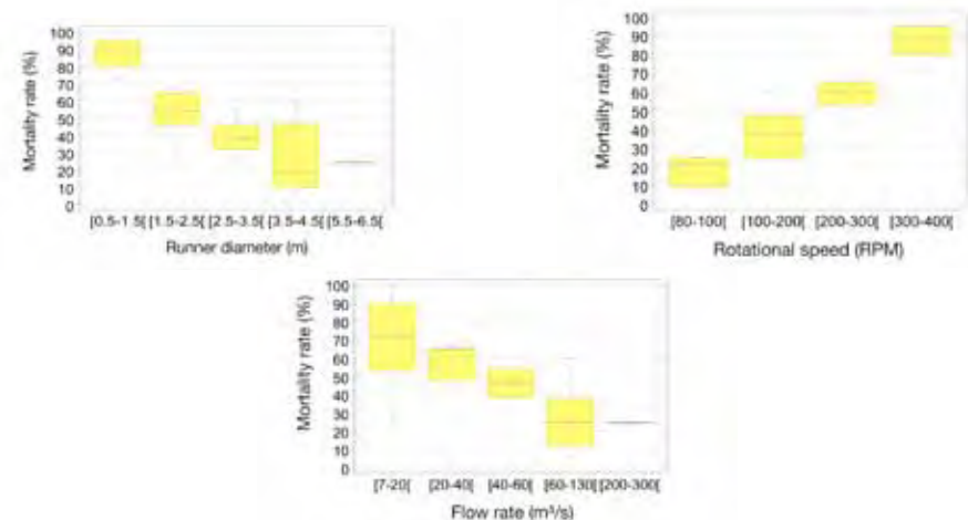
Eel mortality rates while transiting Kaplan turbines as a function of turbine characteristics.
