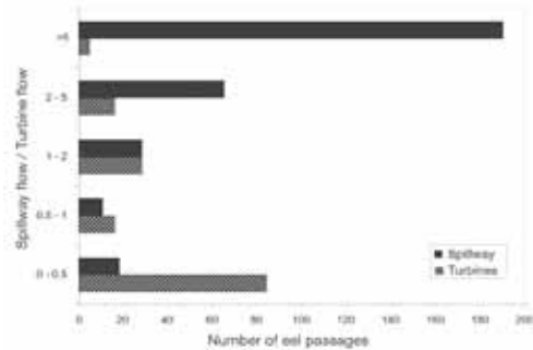
Number of eels passing through the spillways or the turbines as a function of the relative flows via the spillways and the turbines.
