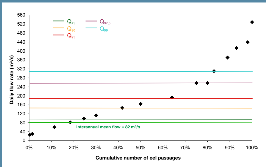
Figure 10. Cumulative passages as a function of the flow rate for six hydroelectric plants on the Gave de Pau river, with selected rated flows.
