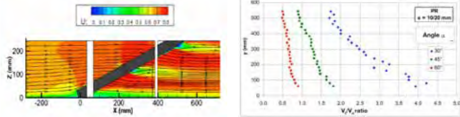
On the left, PIV mapping of longitudinal velocities (m/s) near a screen inclined at an angle of 25^\circ . On the right, the ratio of tangential and normal velocities along angled screens, as a function of the angle.
