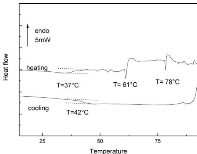
Fig. 1. DSC thermograms of S4 peptides in solution (2 mM) (heating and cooling runs).
