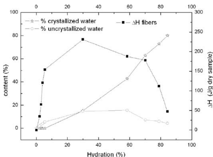
Fig. 8. Amounts of crystallized and uncrystallized water in S4 hydrated fibers and enthalpy of the second endothermic peak as a function of the total hydration of S4 fibres computed from Fig. 7.
