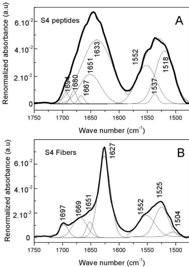
Fig. 3. Decomposed FT-IR spectrum of S4 peptides (A) and S4 fibers (B) in the amide I-II zone (bold line: experimental curve; fine lines: decomposition into Gaussian peaks and sum of the Gaussian peaks).
