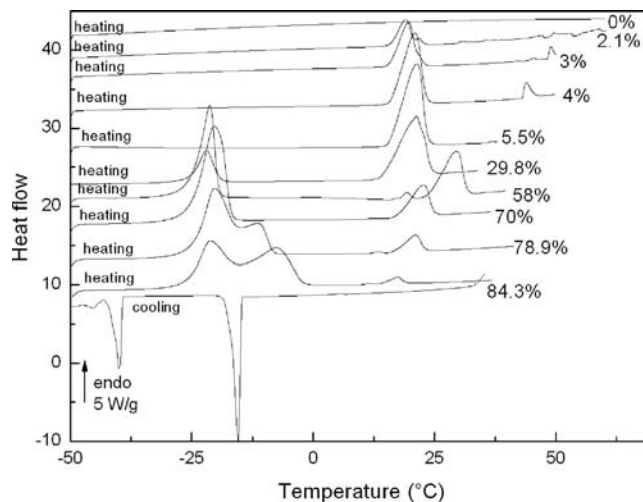
Fig. 7. DSC thermograms of S4 fibers at various hydration levels (cooling and heating runs).
