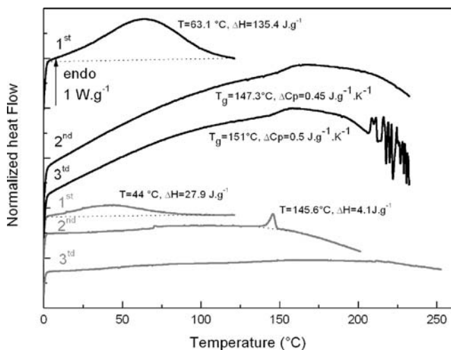
Fig. 6. DSC thermograms of freeze-dried S4 peptides and freeze-dried S4 fibers (first, second and third heating runs).
