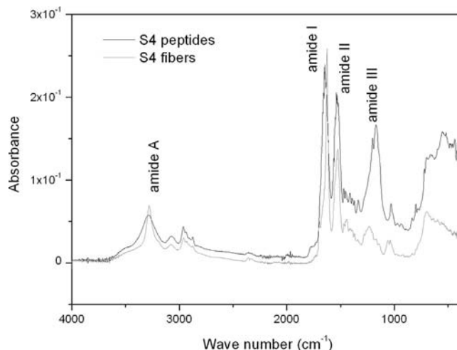
Fig. 2. FT-IR/ATR spectra of freeze-dried S4 peptides and S4 fibres.
