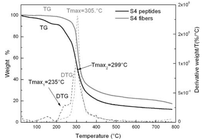
Fig. 4. TGA thermograms (TG) and temperature derivative (DTG) thermograms of freeze-dried S4 peptides and freeze-dried S4 fibres.
