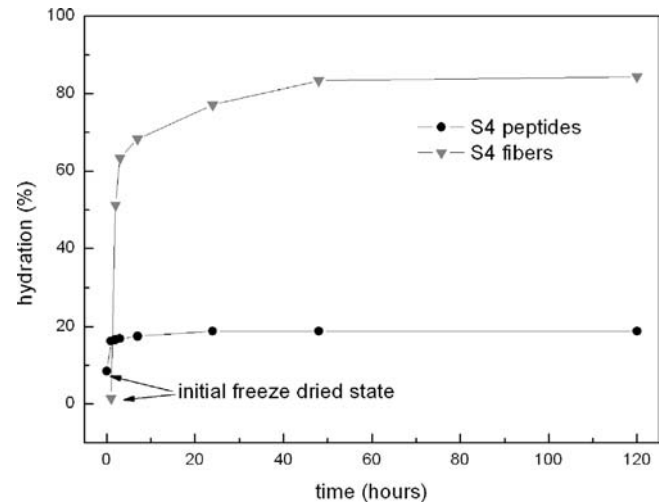
Fig. 5. Water sorption of S4 peptides and S4 fibres under 53% RH at 25 ^{\circ}\text{C} .
