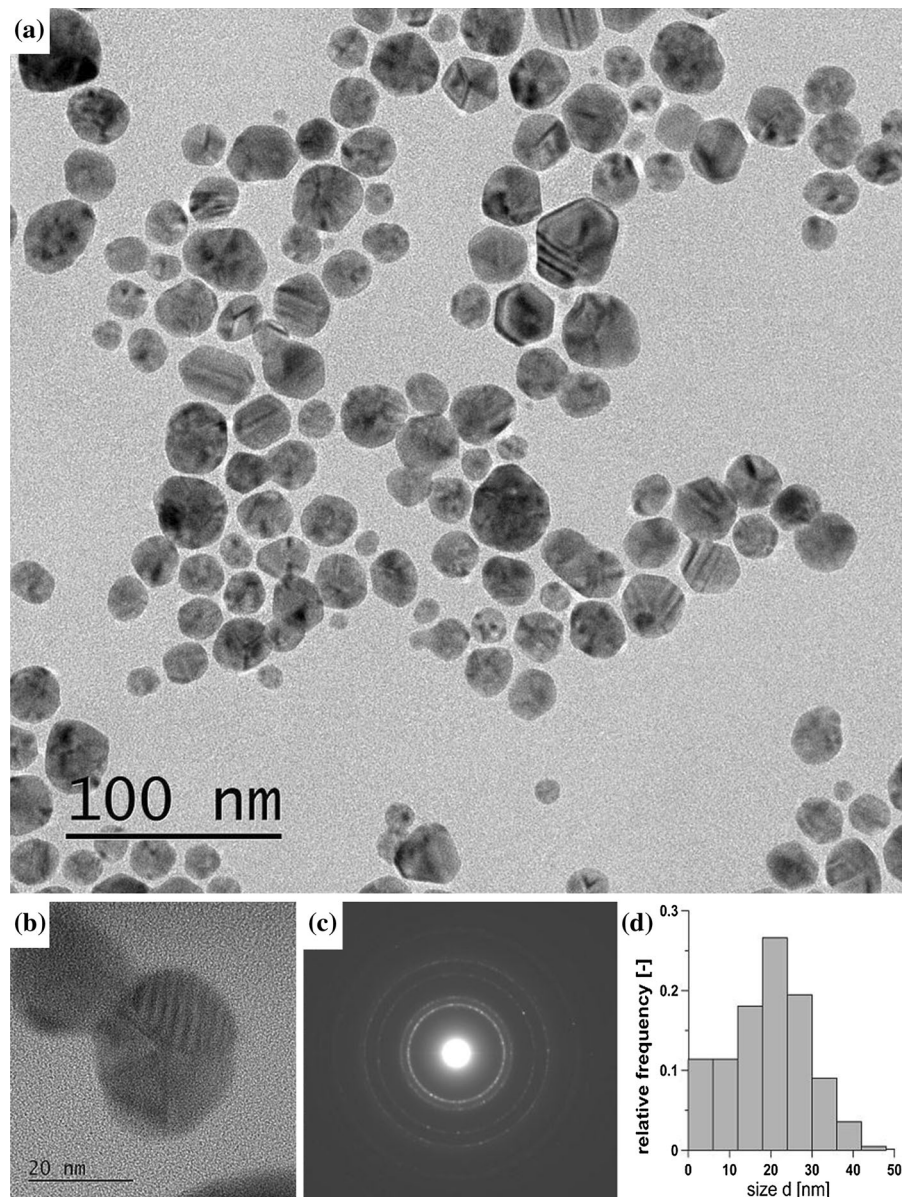
Fig. 7 Characteristics of Ag NPs fabricated in continuous flow process (T14): a TEM image, b HRTEM enlargement, c corresponding SAED pattern, d PSD obtained by counting 420 particles
