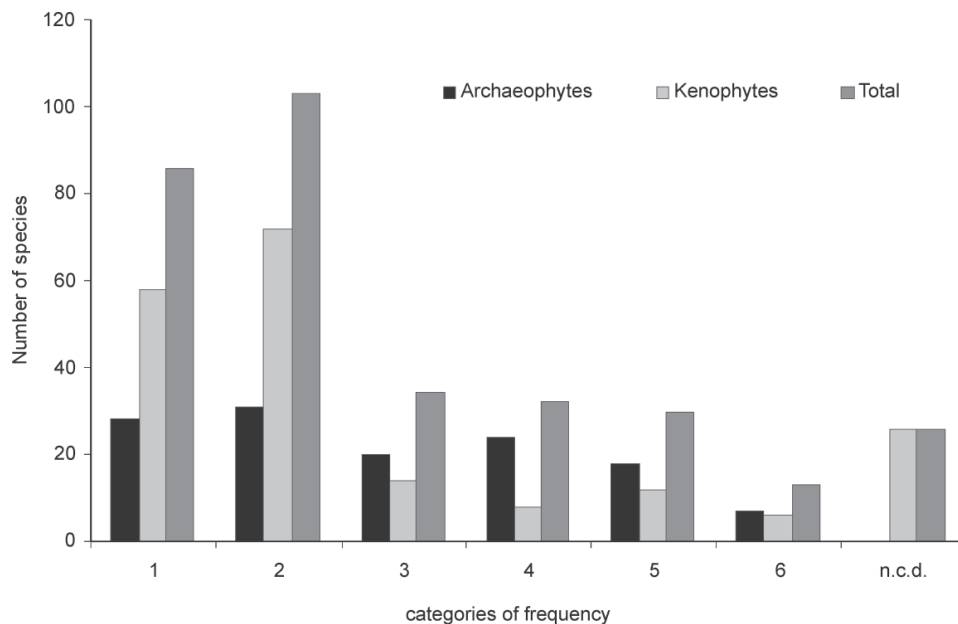
Fig. 7. Frequency distribution of naturalized alien flora in the Silesian Upland Explanations: categories of frequency, 1 – rare, 2 – occasional, 3 – occasional, locally frequent, 4 – frequent, locally abundant, 5 – abundant, 6 – common; for more explanation see chapter 2
