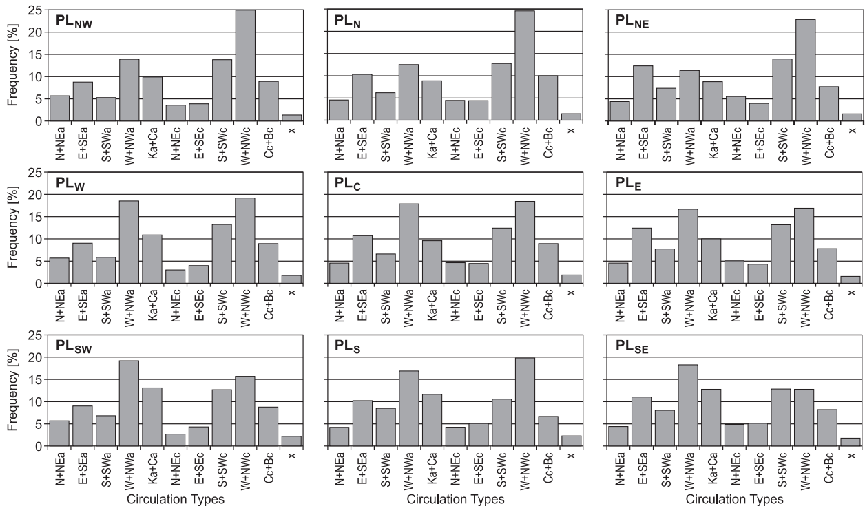
Fig. 2. Frequency of circulation types in winter (DJF) for grid box within Poland. PL_{NW} , PL_N , ... etc. – grid box within Poland, e.g.: PL_{NW} – North-western grid box (see Fig. 1)
