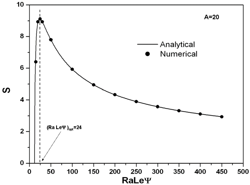
Figure 7: Separation ( S ) versus (Ra Le \Psi) .
