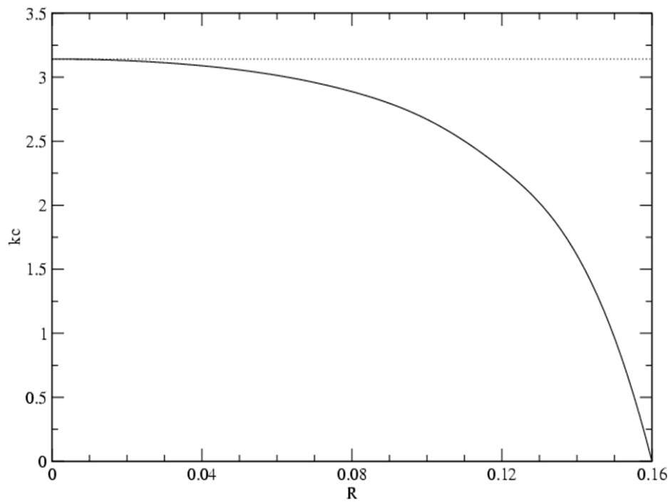
Figure 2: Influence of vibration parameter on the critical wave number k_c (Darcy model) for the layer heated from below.
