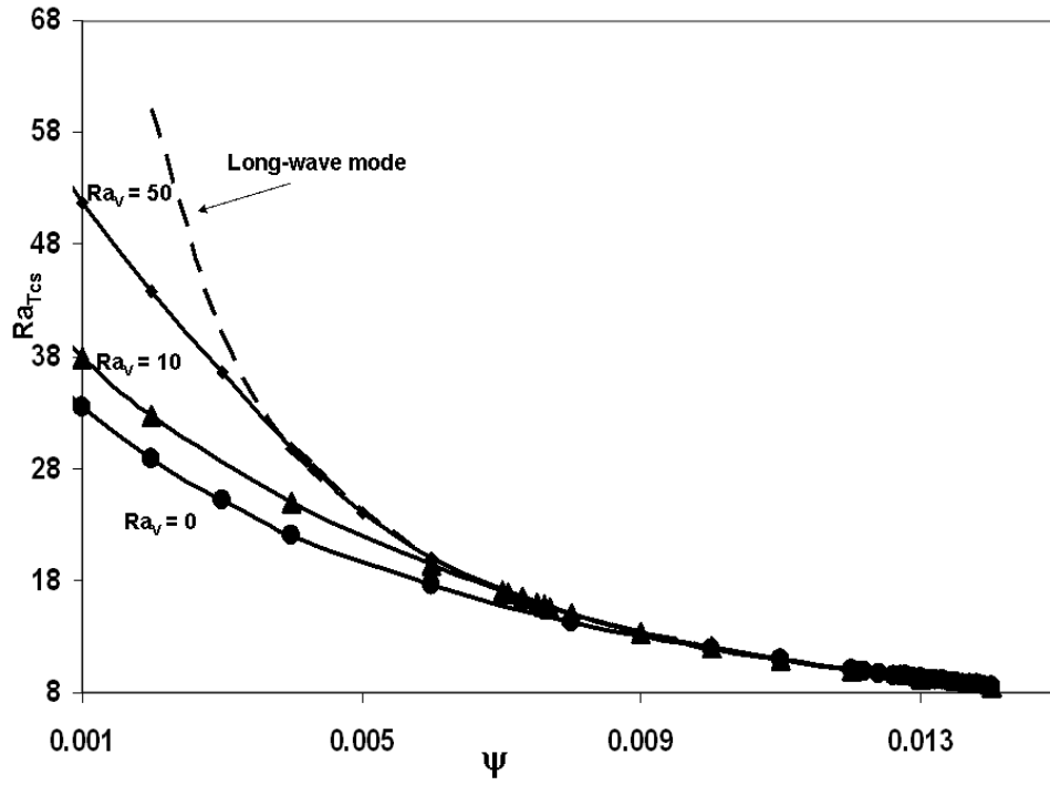
Figure 4: Effect of vertical vibration on the onset Soret-driven convection, Le = 100 , \varepsilon^* = 0.5 and B = 10^{-6} for the layer heated from below.
