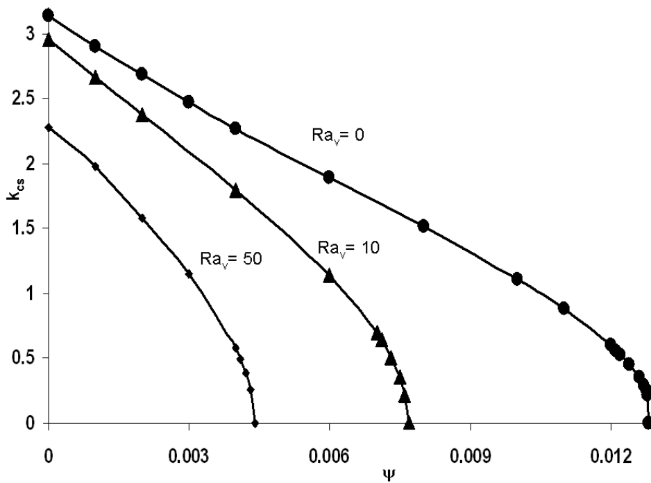
Figure 5: Effect of vertical vibration on the critical wave number in Soret-driven convection, Le = 100 , \varepsilon^* = 0.5 and B = 10^{-6} for the layer heated from below
