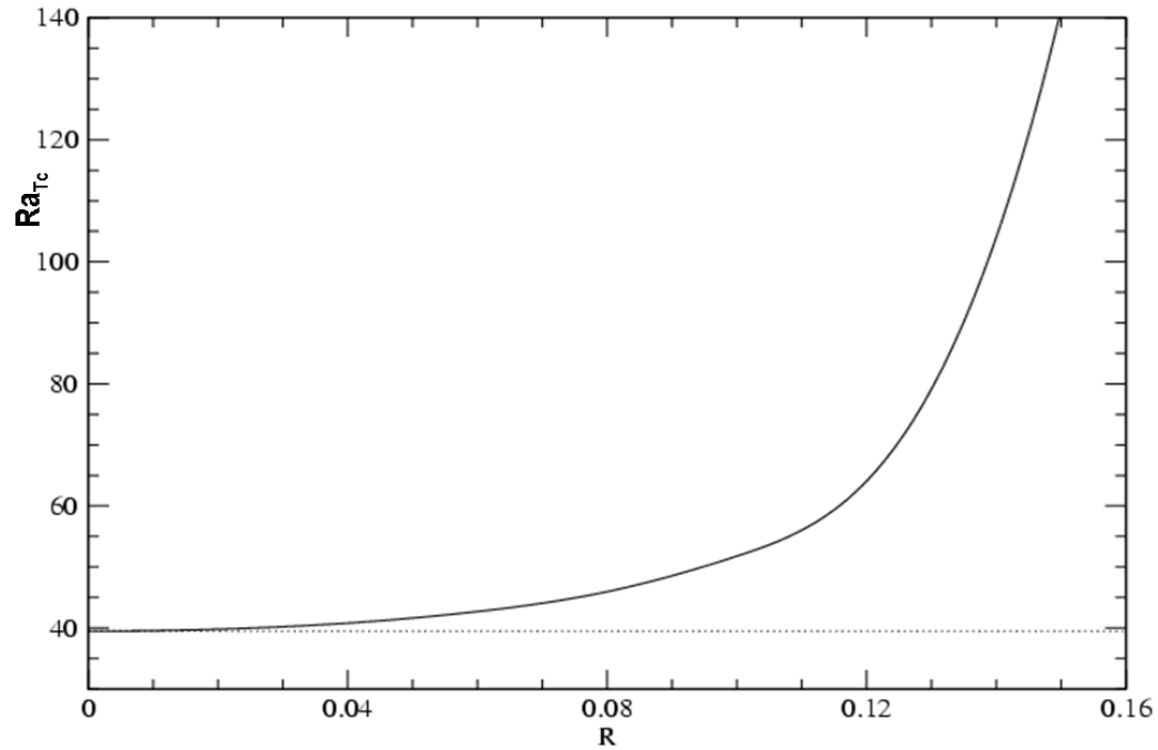
Figure 1: Influence of vertical vibration parameter R on the onset of convection in a horizontal porous layer saturated by a pure fluid (Darcy model) for the layer heated from below.
