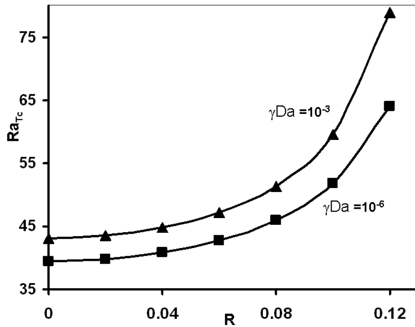
Figure 3: Influence of vertical vibration on the critical Rayleigh number for different values of \gamma Da for the layer heated from below.
