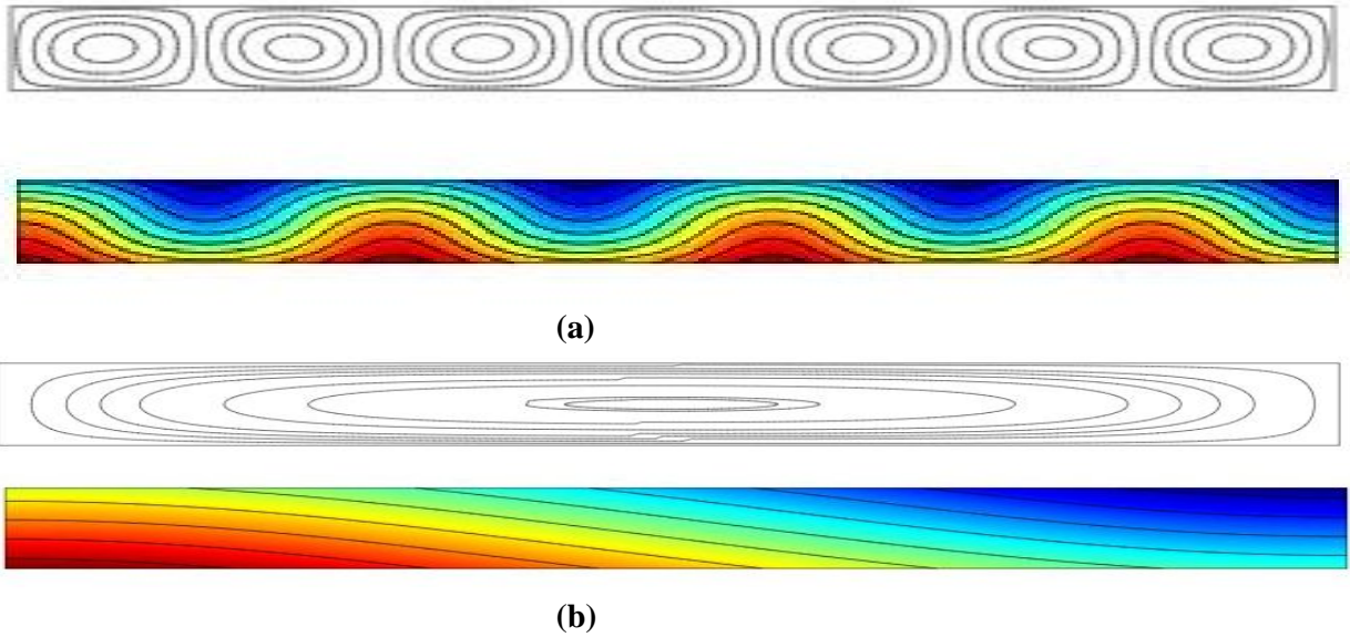
Figure 8: Streamlines and iso-concentrations a) Static gravity ( Ra_v = 0 ) b) simultaneous effects of vibration and gravitation ( Ra_v = 20 ), Ra_T = 15.7 , Le = 2 , A = 10 and \epsilon^* = 0.5
