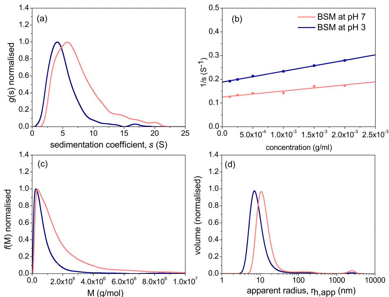
Fig. 3 Comparative hydrodynamic properties of bovine submaxillary mucin at pH 7.0 and at pH 3.0 (a) sedimentation coefficient g(s) distribution at 0.25 mg/ml; b reciprocal plot of s versus concentration, fitted to (1/s) = (1/s^\circ)(1 + k_s c) where k_s is the concentration dependence ‘Gralén’ coefficient [47]; c molecular weight distribution from
