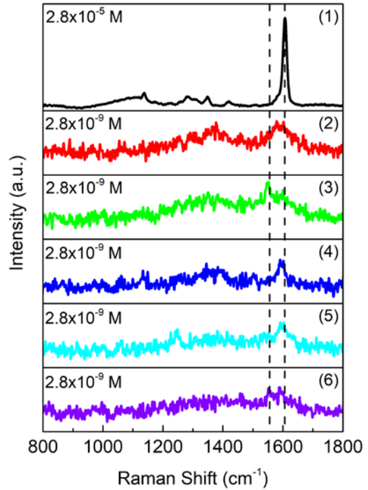
Figure 5. Raman spectra from F8-PFB at 2.8 \times 10^{-5} M on glass (panel 1), and SERS spectra from F8-PFB at 2.8 \times 10^{-9} M within the nano-gaps between a silver nanoparticle and silver film (panels 2-6).
