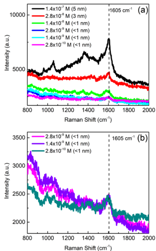
Figure 3. SERS concentration study of F8-PFB for 118 nm silver nanoparticles on a silver film (estimated thickness in parentheses) taken at 532 nm excitation with 3 s collection time. (a) The full concentration range and (b), the point at which intensity no longer drops.
