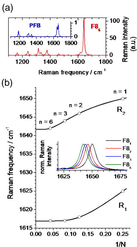
Figure 6. DFT calculations demonstrating (a) Raman spectrum of F8 6 (PFB as inset). (b) Peak shift of R 1 and R 2 Raman frequencies towards the polymer limit ( N^{-1} = 0 ; see Method section).
