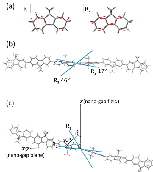
Figure 7. (a) Relative atomic displacements of the C-atoms in the central fluorene units for R 1 and R 2 . (b) Main axis of the polarizability tensor of R 1 and R 2 for F8 6 : (angles vs. terminal C-C). (c) Orientation of the target analyte with respect to the nano-gap field.
