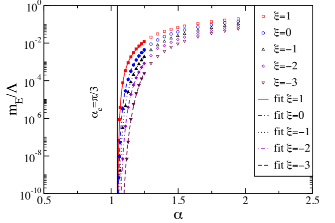
FIG. 3: Ratio of the Euclidean mass and the ultraviolet cut-off in different gauges. \alpha_c = \pi/3 within the numerical accuracy of our computation.
