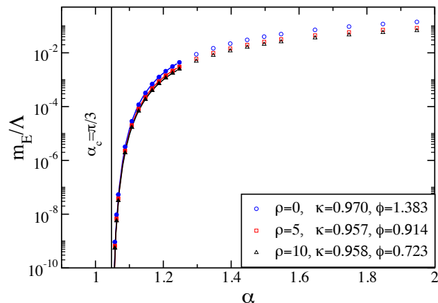
FIG. 4: Euclidean mass in Landau gauge for \rho = 0, 5, 10 . \rho stands for the strength of the DCSB in the vertex, Eq. (146)
