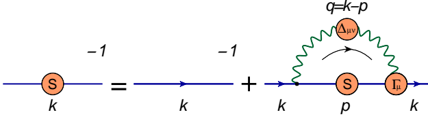
FIG. 2: Gap equation for the fermion propagator. The color-filled blobs labelled with S , \Delta_{\mu\nu} and \Gamma_\mu stand for the fully-dressed fermion and photon propagators, and the three-point vertex, respectively.
