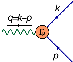
FIG. 1: Diagrammatic representation of the full three-point vertex \Gamma_\mu(k, p) , with momentum flow indicated.
