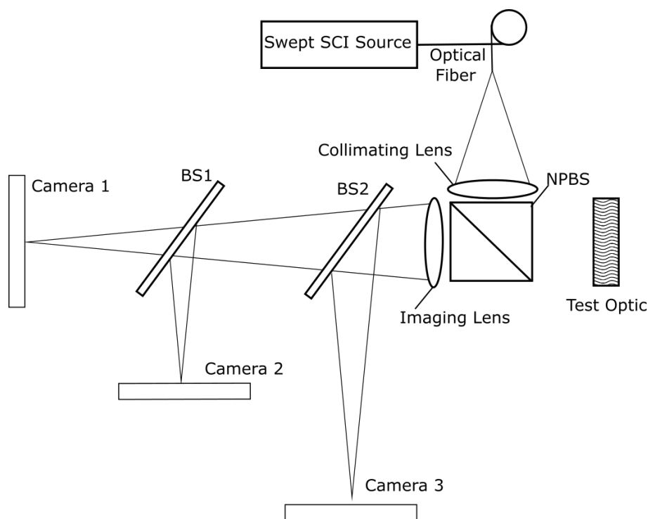
Figure 6. Experimental diagram for 3 camera non-polarization based Fizeau interferometer with scanning SCI source. No transmission flat is used in the experiment, and internal fringes of the plane parallel plate are produced and measured. BS : Beam splitter. NPBS: Non polarizing beam splitter cube.
