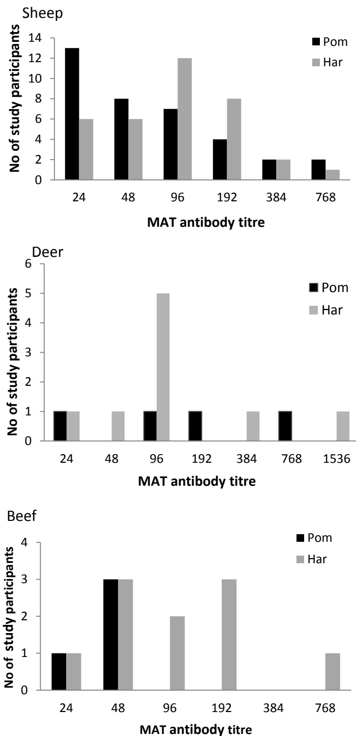
Figure 2. Frequency histogram showing the number of sero-positive study participants at each MAT titre to serovars Leptospira interrogans sv. Pomona (black) and Leptospira borgpetersenii sv. Hardjovovis (grey) in sheep (top), deer (middle) and beef abattoirs (bottom).
