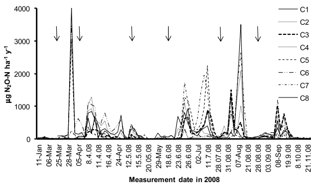
Figure 5. Spatial and temporal variability of N 2 O fluxes measured by eight static chambers (C1–C8) from a grazed grassland in the UK (Skiba et al 2013). The arrows denote dates of N fertilizer application (52 kg N ha -1 yr -1 in March, May, June, July, 69 kg N ha -1 yr -1 in April and 35 kg N ha -1 yr -1 in August). The onset and magnitude of fertilizer induced N 2 O emission peaks was different for each chamber and each fertilizer event.
