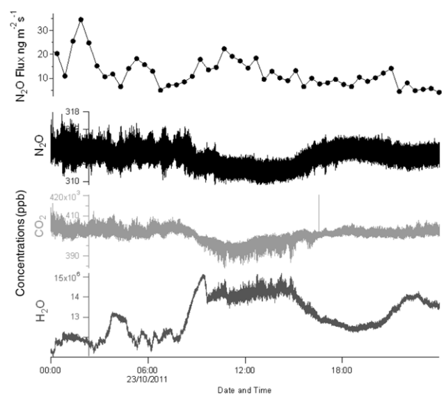
Figure 8. An example day of mixing ratios (1 ppb = 1 ng l -1 ) of N 2 O, CO 2 and H 2 O recorded at 10 Hz by the QCL (three bottom traces), and calculated N 2 O fluxes (top trace). These measurements were made from a grassland in England fertilized with slurry.
