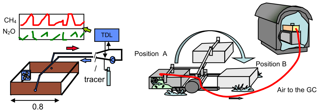
Figure 6. Two chamber methods setups used to overcome the spatial and temporal variability problems associated with soil N 2 O fluxes. The fast chamber method (left), using the TDL or QCL as a sensor, allows many measurements at different locations in a short period of time. On the right the automatic chamber that alternates between two positions and is connected to a GC and enables many measurements from the same locations throughout a day.
