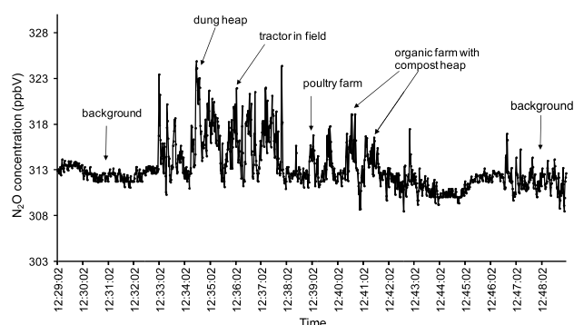
Figure 10. Typical trace of mobile plume measurements in an agricultural area using a TDL to detect N 2 O fluxes at 10 Hz recorded in spring on a 33 ha flat region in UK, containing crops, a small poultry farm, dung heaps and an organic farm. The average concentration increase was 2.6 \pm 2.7 ppb (1 ppb = 1 ng l -1 ). Results suggest that for this period the N 2 O emission rate was 290 ng N 2 O m -2 s -1 .
