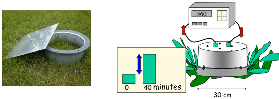
Figure 4. Chamber measurement methods measure the increasing (or decreasing) concentration inside a chamber, preferably a number of times after closing the chamber. The photo on the left is of a low cost static manual chamber, made from commercially available drainpipe (40 cm diameter), flange and an aluminum lid and used for manual sampling of the air into glass vials for subsequent analysis by gas chromatography (figure 2). The schematic diagram on the right shows a chamber connected to a photo-acoustic analyzer, the air is re-circulated between analyzer and instrument, and the increase in N 2 O concentration is measured once a minute. CO 2 and H 2 O have to be scrubbed from the gas flow in order to get useful N 2 O data.
