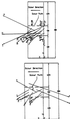
Figure 4.10. (Top) Post-test displacement of bivalves at the sediment/water interface ( z = 500 ) in RB1. Cyclocardia sp. A: 1 (12.3 mm), 2 (13.3 mm), 3 (17.8 mm), 4 (23.4 mm), 5 (17.0 mm), 6 (21.4 mm), 7 (21.8 mm); Astarte borealis : 8 (37.5 mm), 9 (37.0 mm), 10 (35.8 mm), 11 (40.9 mm), 12 (40.0 mm), 13 (38.3 mm), 14 (34.7 mm), 15 (35.6 mm), 16 (37.0 mm); Clinocardium ciliatum : 17 (15.0 mm), 18 (14.4 mm), 19 (55.6 mm); Cyclocardia novangliae : 20 (15.6 mm), 21 (17.3 mm), 22 (17.8 mm), 23 (17.3 mm), 24 (17.5 mm), 25 (18.0 mm), 26 (19.3 mm). (Bottom) Post-test displacement of bivalves at the sediment/water interface ( z = 500 ) in RB2. Astarte borealis : 1 (40.0 mm), 2 (36.1 mm), 3 (41.2 mm); Clinocardium ciliatum : 4 (14.0 mm), 5 (12.7 mm), 6 (55.0 mm), 7 (54.9 mm); Macoma calcarea : 8 (11.4 mm), 9 (12.7 mm), 10 (15.2 mm), 11 (13.0 mm), 12 (13.0 mm), 13 (15.1 mm).
