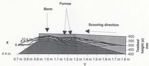
Figure 4.6. Post-scour testbed profile.
