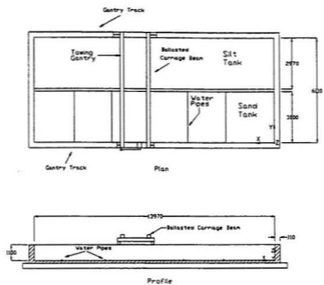
Figure 4.1. Plan and profile views of the experimental tank used for the trawl door model experiment (dimensions in mm).
